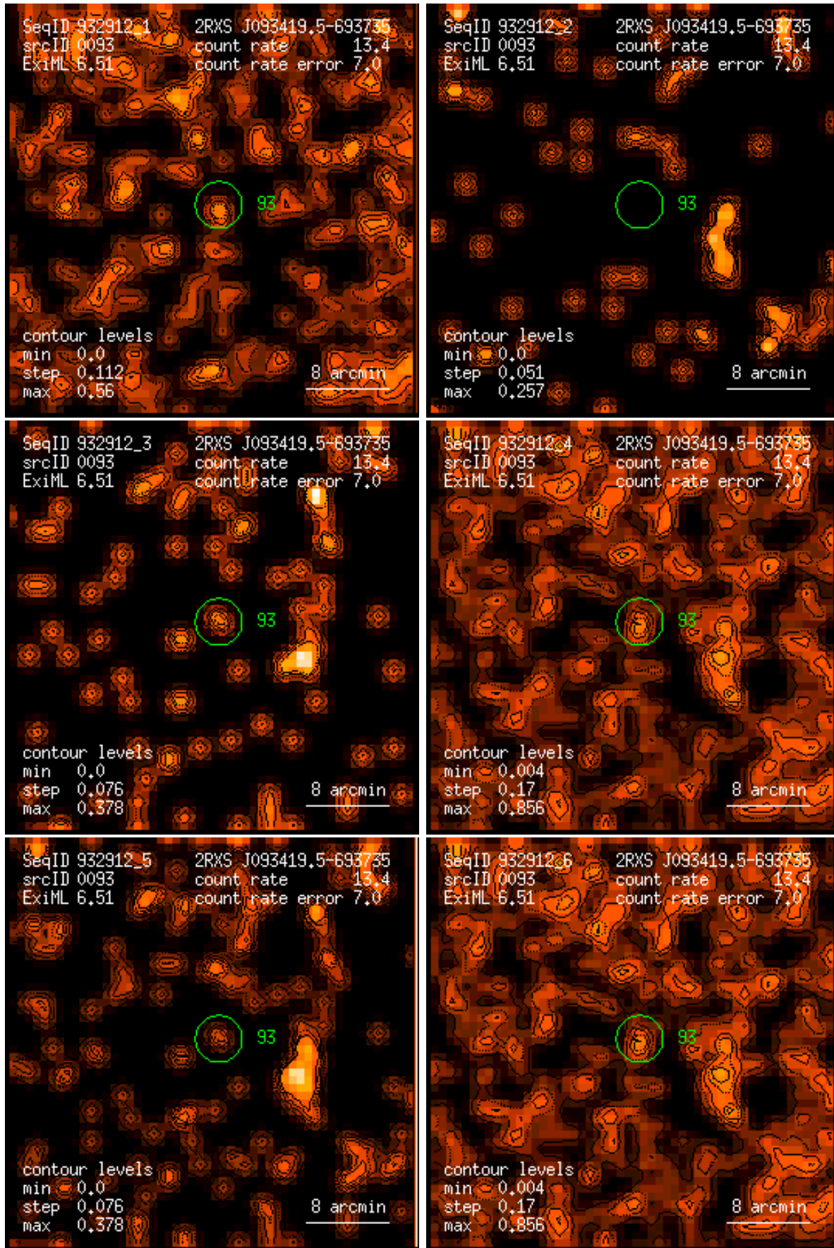
Figure 93: RASS 932912: detection 0093: band rate images, Gaussian filter: (1) PSPC channels 11 – 41, (2) 52 – 90, (3) 91 – 201, (4) 11 – 235, (5) 52 – 201, (6) 11 – 201. Broad band rates in counts/ks. Band rate contour levels in counts/ks/arcmin 2 .
