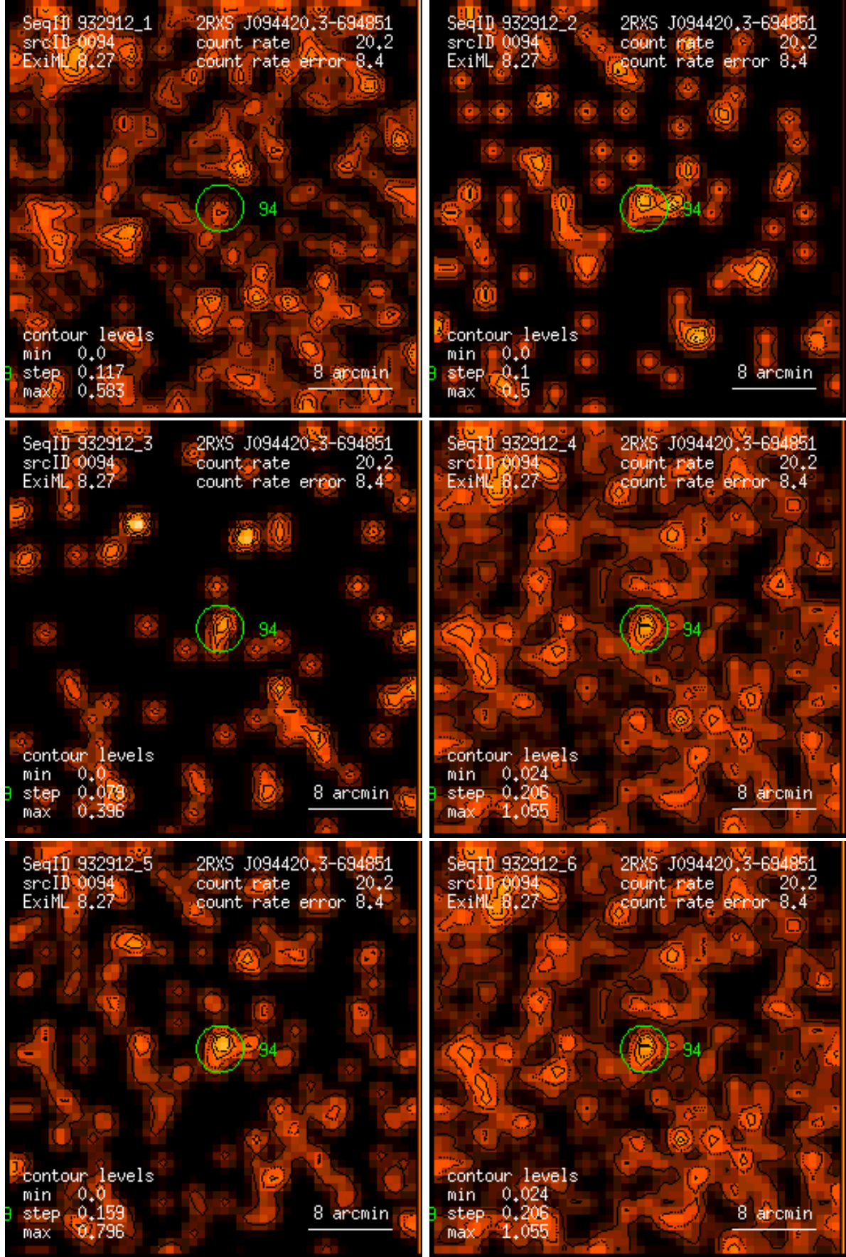
Figure 94: RASS 932912: detection 0094: band rate images, Gaussian filter: (1) PSPC channels 11 – 41, (2) 52 – 90, (3) 91 – 201, (4) 11 – 235, (5) 52 – 201, (6) 11 – 201. Broad band rates in counts/ks. Band rate contour levels in counts/ks/arcmin 2 .
