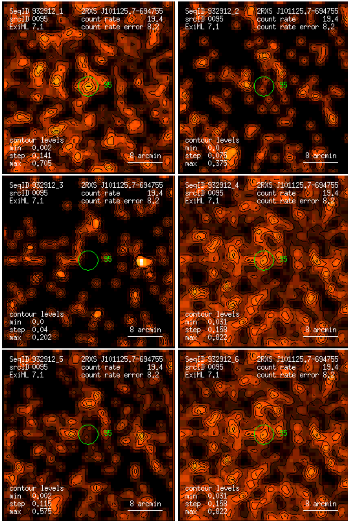
Figure 95: RASS 932912: detection 0095: band rate images, Gaussian filter: (1) PSPC channels 11 – 41, (2) 52 – 90, (3) 91 – 201, (4) 11 – 235, (5) 52 – 201, (6) 11 – 201. Broad band rates in counts/ks. Band rate contour levels in counts/ks/arcmin 2 .
