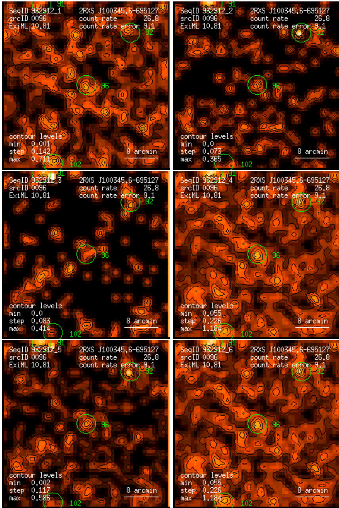
Figure 96: RASS 932912: detection 0096: band rate images, Gaussian filter: (1) PSPC channels 11 – 41, (2) 52 – 90, (3) 91 – 201, (4) 11 – 235, (5) 52 – 201, (6) 11 – 201. Broad band rates in counts/ks. Band rate contour levels in counts/ks/arcmin 2 .
