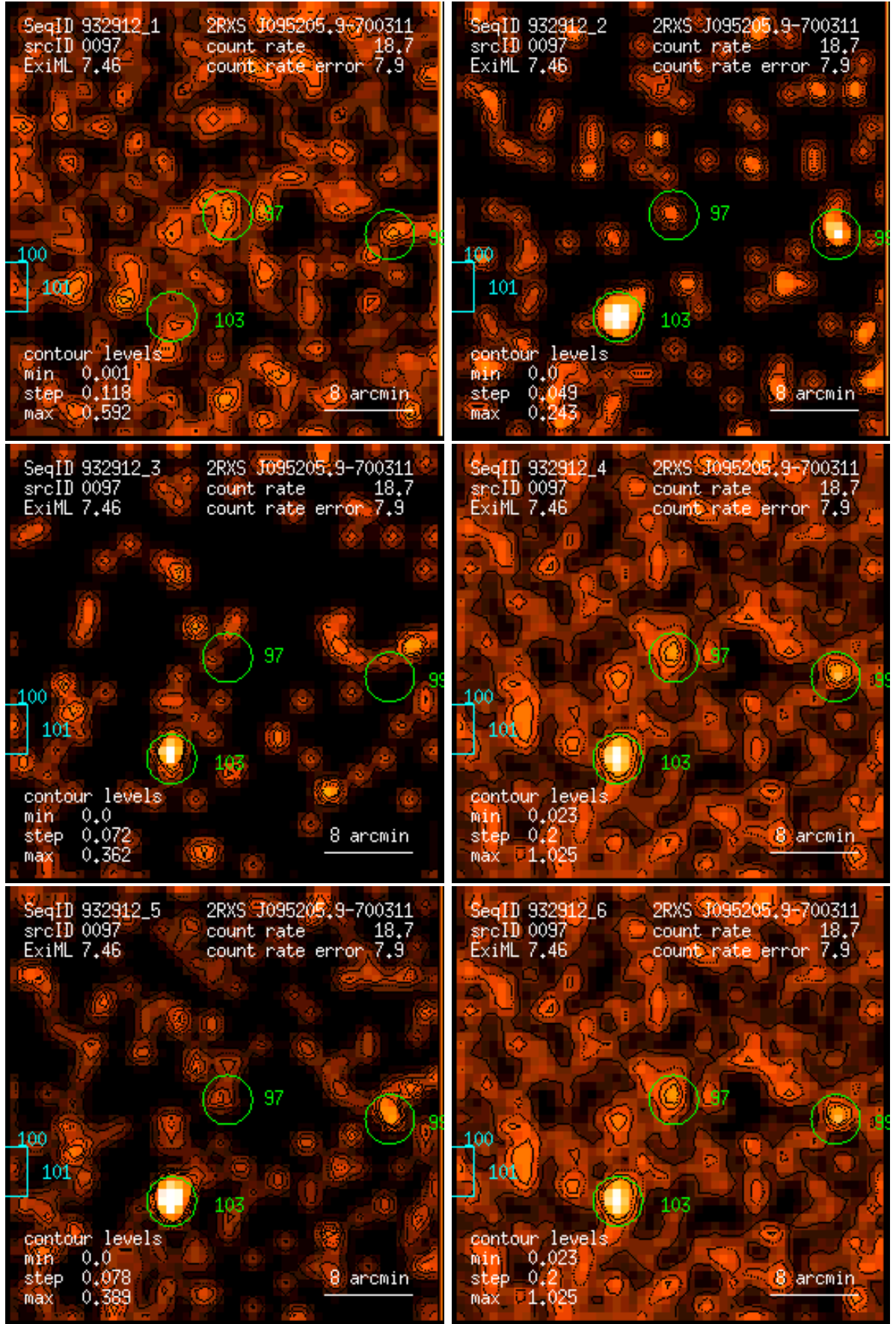
Figure 97: RASS 932912: detection 0097: band rate images, Gaussian filter: (1) PSPC channels 11 – 41, (2) 52 – 90, (3) 91 – 201, (4) 11 – 235, (5) 52 – 201, (6) 11 – 201. Broad band rates in counts/ks. Band rate contour levels in counts/ks/arcmin 2 .
