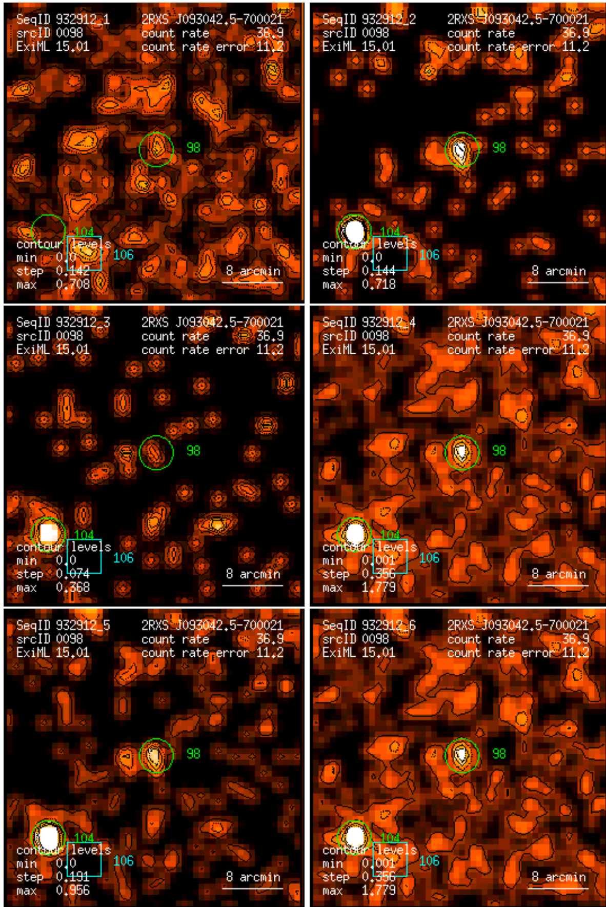
Figure 98: RASS 932912: detection 0098: band rate images, Gaussian filter: (1) PSPC channels 11 – 41, (2) 52 – 90, (3) 91 – 201, (4) 11 – 235, (5) 52 – 201, (6) 11 – 201. Broad band rates in counts/ks. Band rate contour levels in counts/ks/arcmin 2 .
