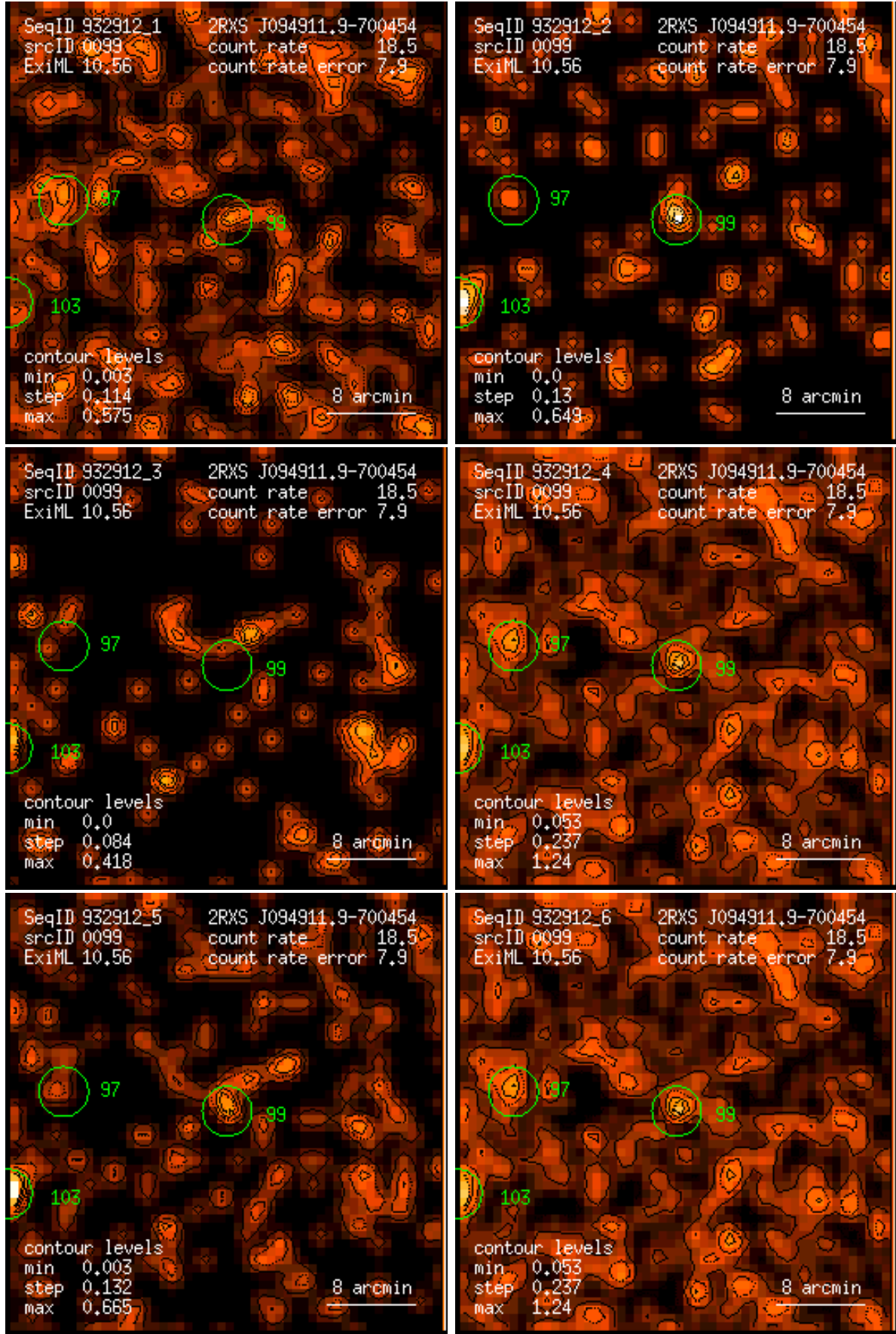
Figure 99: RASS 932912: detection 0099: band rate images, Gaussian filter: (1) PSPC channels 11 – 41, (2) 52 – 90, (3) 91 – 201, (4) 11 – 235, (5) 52 – 201, (6) 11 – 201. Broad band rates in counts/ks. Band rate contour levels in counts/ks/arcmin 2 .
