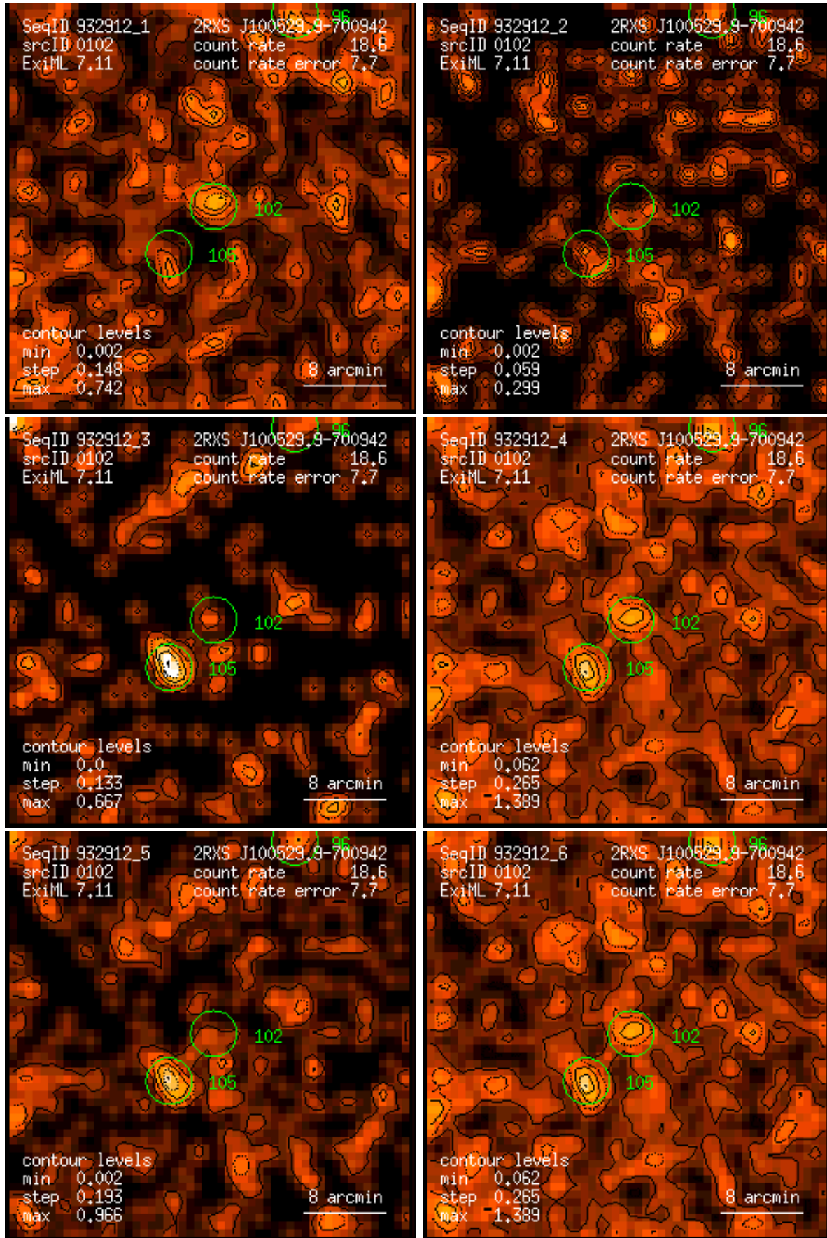
Figure 102: RASS 932912: detection 0102: band rate images, Gaussian filter: (1) PSPC channels 11 – 41, (2) 52 – 90, (3) 91 – 201, (4) 11 – 235, (5) 52 – 201, (6) 11 – 201. Broad band rates in counts/ks. Band rate contour levels in counts/ks/arcmin 2 .
