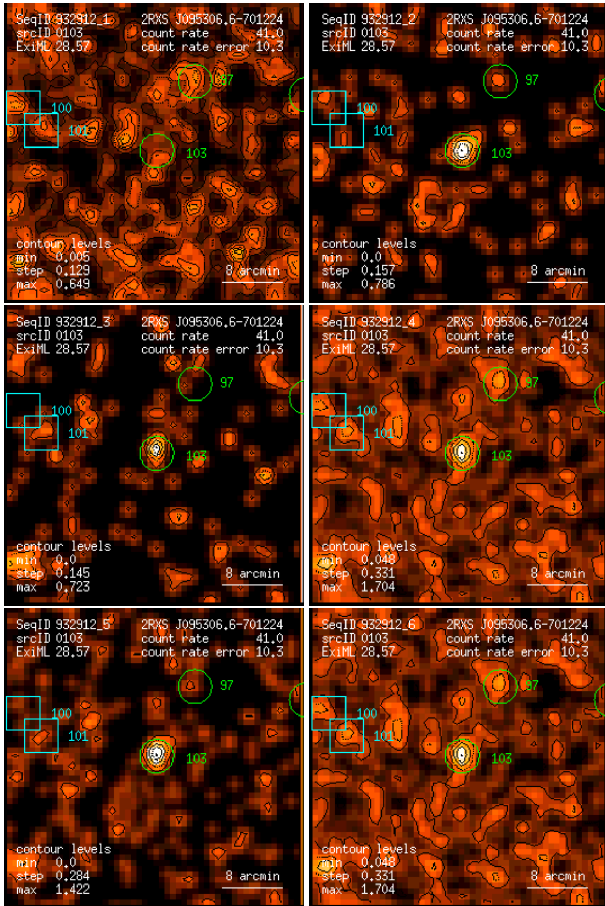
Figure 103: RASS 932912: detection 0103: band rate images, Gaussian filter: (1) PSPC channels 11 – 41, (2) 52 – 90, (3) 91 – 201, (4) 11 – 235, (5) 52 – 201, (6) 11 – 201. Broad band rates in counts/ks. Band rate contour levels in counts/ks/arcmin 2 .
