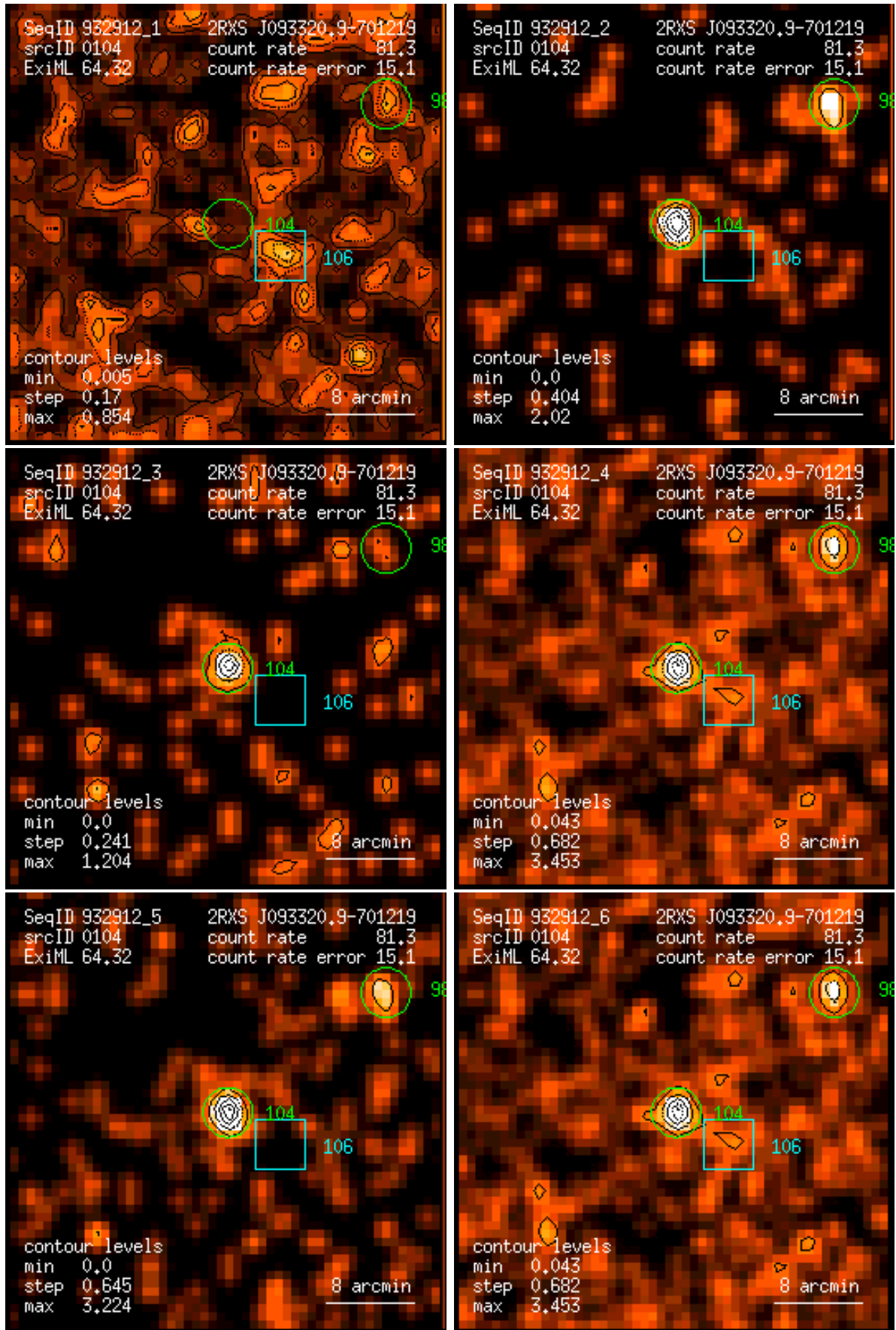
Figure 104: RASS 932912: detection 0104: band rate images, Gaussian filter: (1) PSPC channels 11 – 41, (2) 52 – 90, (3) 91 – 201, (4) 11 – 235, (5) 52 – 201, (6) 11 – 201. Broad band rates in counts/ks. Band rate contour levels in counts/ks/arcmin 2 .
