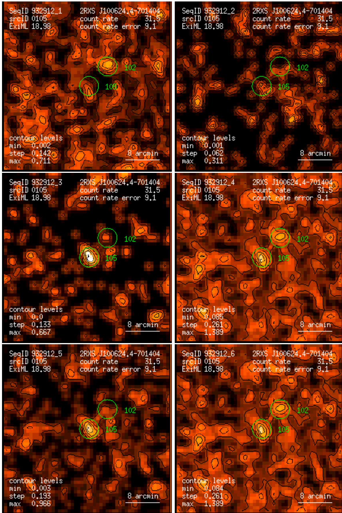
Figure 105: RASS 932912: detection 0105: band rate images, Gaussian filter: (1) PSPC channels 11 – 41, (2) 52 – 90, (3) 91 – 201, (4) 11 – 235, (5) 52 – 201, (6) 11 – 201. Broad band rates in counts/ks. Band rate contour levels in counts/ks/arcmin 2 .
