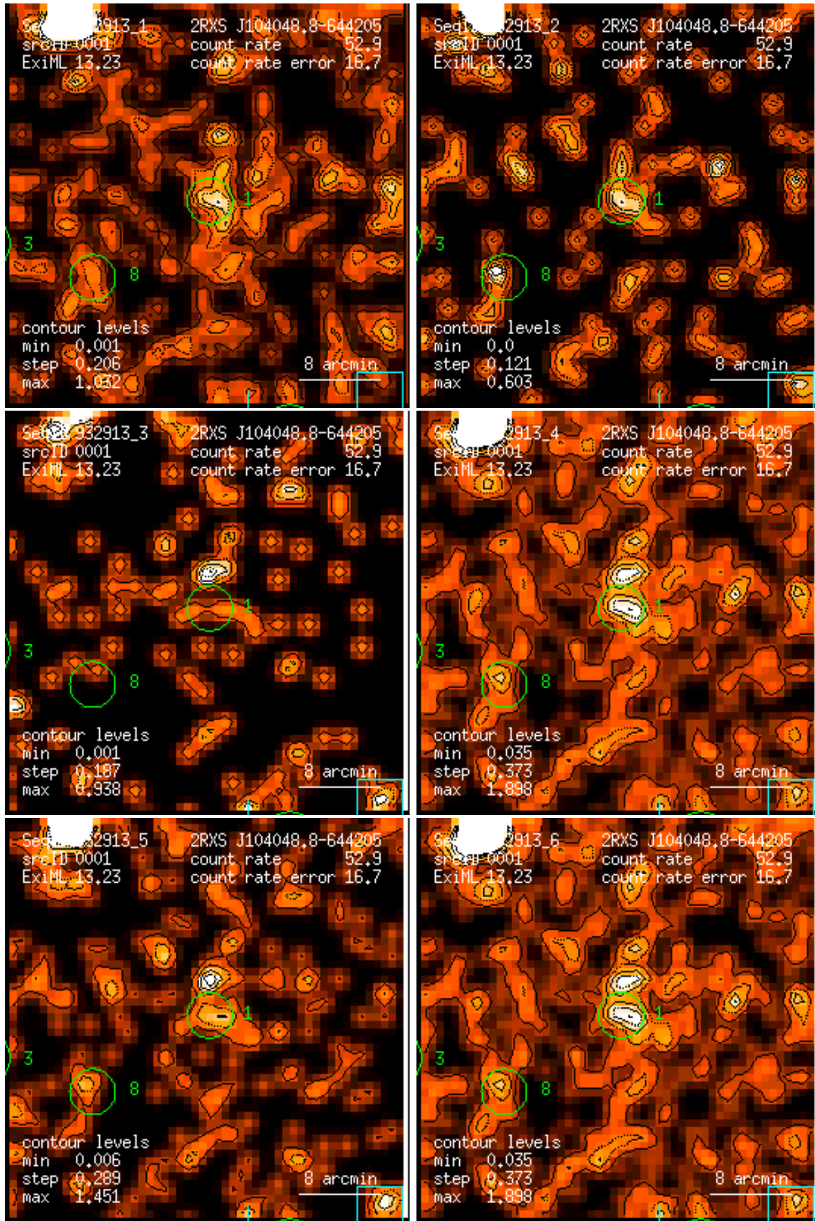
Figure 1: RASS 932913: detection 0001: band rate images, Gaussian filter: (1) PSPC channels 11 – 41, (2) 52 – 90, (3) 91 – 201, (4) 11 – 235, (5) 52 – 201, (6) 11 – 201. Broad band rates in counts/ks. Band rate contour levels in counts/ks/arcmin 2 .
