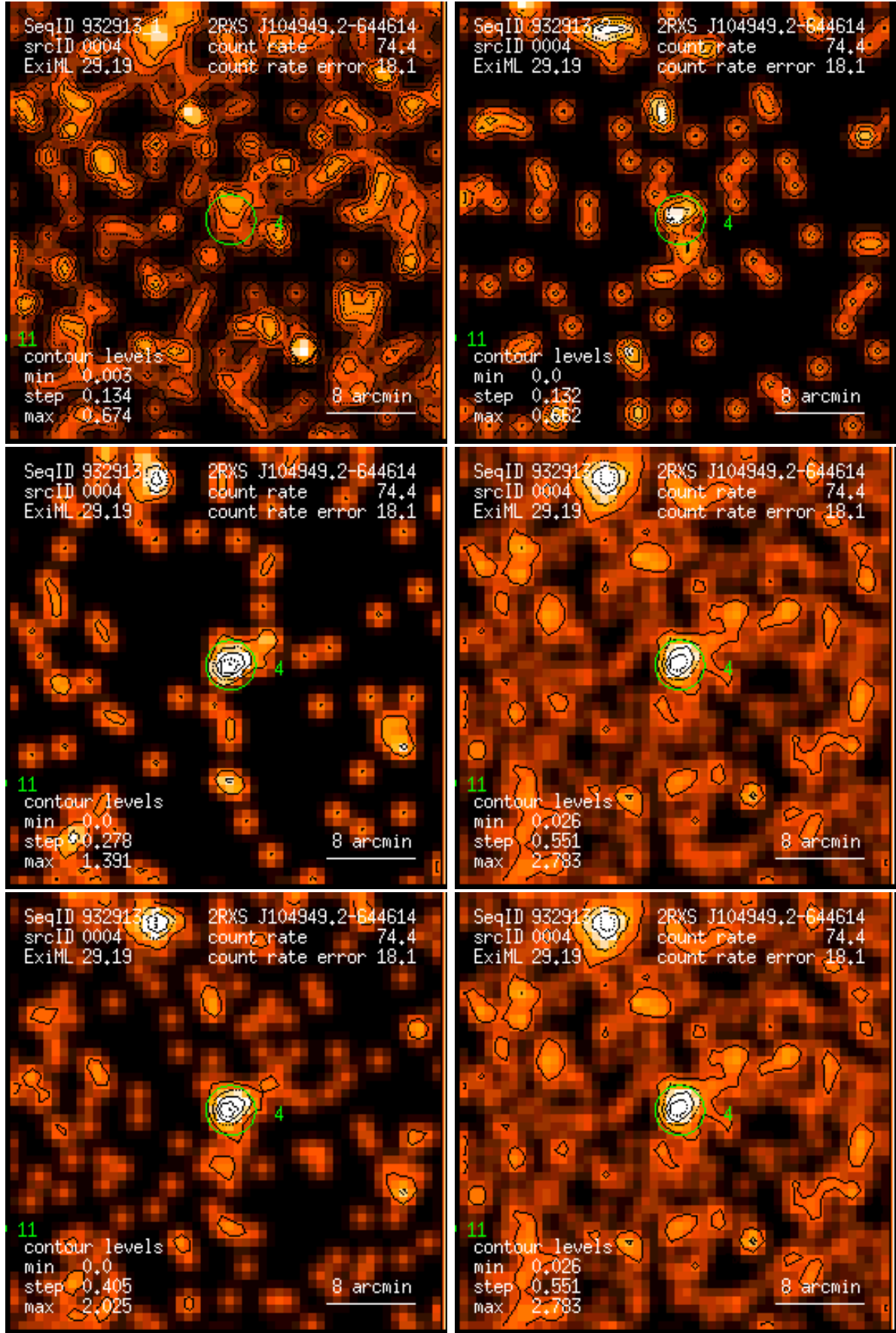
Figure 4: RASS 932913: detection 0004: band rate images, Gaussian filter: (1) PSPC channels 11 – 41, (2) 52 – 90, (3) 91 – 201, (4) 11 – 235, (5) 52 – 201, (6) 11 – 201. Broad band rates in counts/ks. Band rate contour levels in counts/ks/arcmin 2 .
