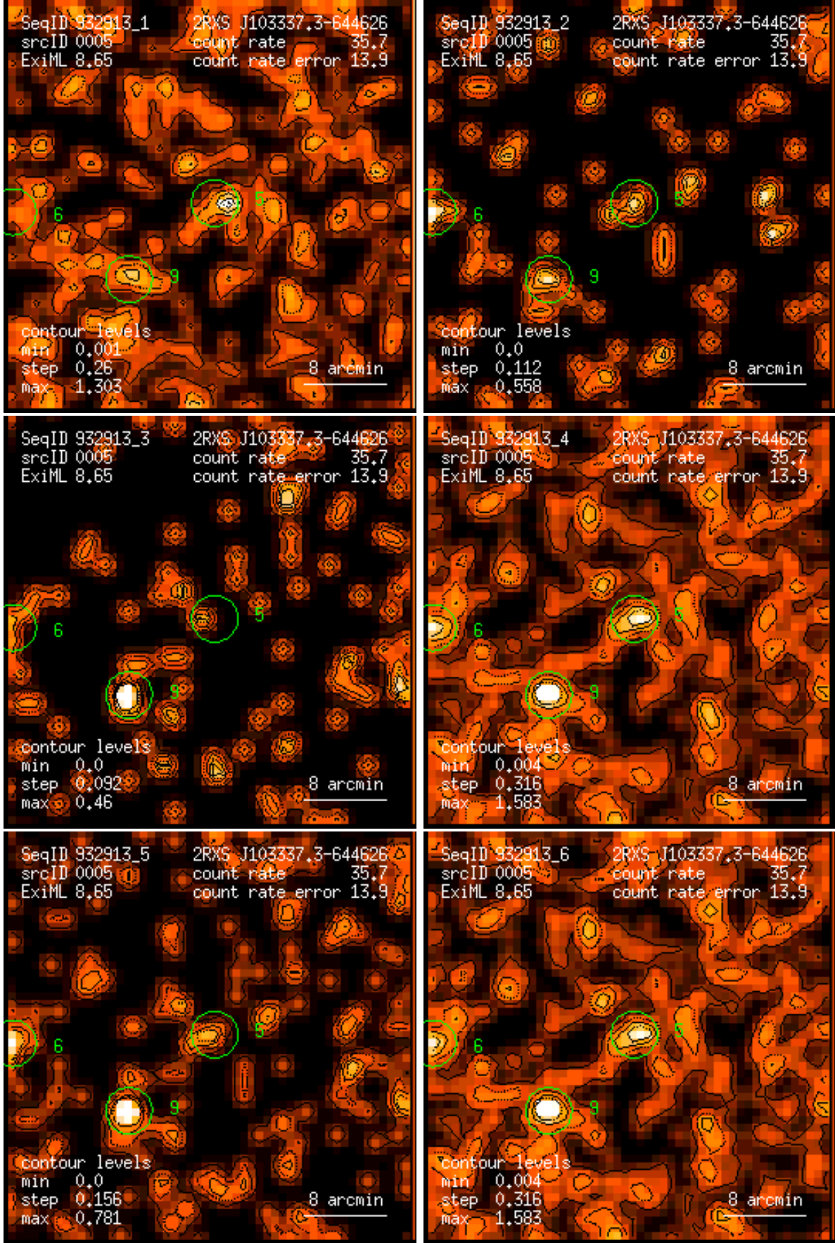
Figure 5: RASS 932913: detection 0005: band rate images, Gaussian filter: (1) PSPC channels 11 – 41, (2) 52 – 90, (3) 91 – 201, (4) 11 – 235, (5) 52 – 201, (6) 11 – 201. Broad band rates in counts/ks. Band rate contour levels in counts/ks/arcmin 2 .
