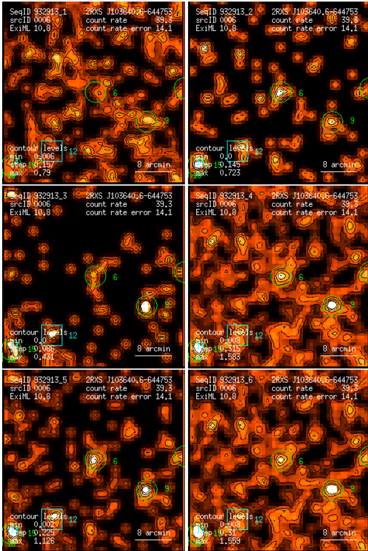
Figure 6: RASS 932913: detection 0006: band rate images, Gaussian filter: (1) PSPC channels 11 – 41, (2) 52 – 90, (3) 91 – 201, (4) 11 – 235, (5) 52 – 201, (6) 11 – 201. Broad band rates in counts/ks. Band rate contour levels in counts/ks/arcmin 2 .
