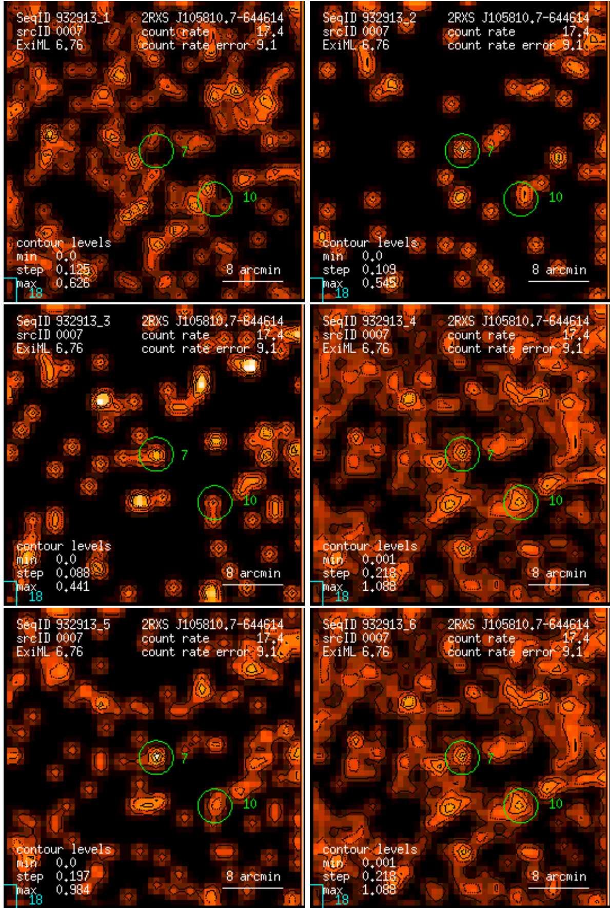
Figure 7: RASS 932913: detection 0007: band rate images, Gaussian filter: (1) PSPC channels 11 – 41, (2) 52 – 90, (3) 91 – 201, (4) 11 – 235, (5) 52 – 201, (6) 11 – 201. Broad band rates in counts/ks. Band rate contour levels in counts/ks/arcmin 2 .
