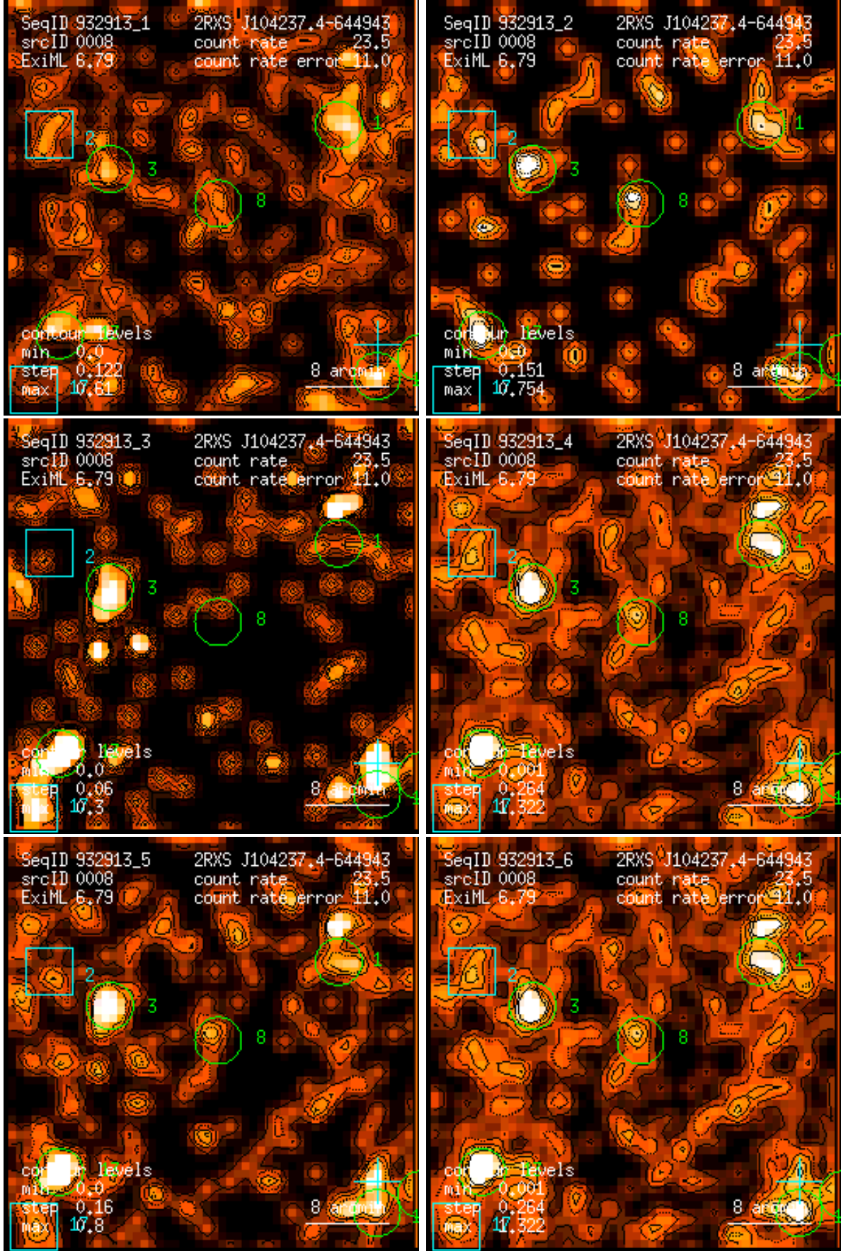
Figure 8: RASS 932913: detection 0008: band rate images, Gaussian filter: (1) PSPC channels 11 – 41, (2) 52 – 90, (3) 91 – 201, (4) 11 – 235, (5) 52 – 201, (6) 11 – 201. Broad band rates in counts/ks. Band rate contour levels in counts/ks/arcmin 2 .
