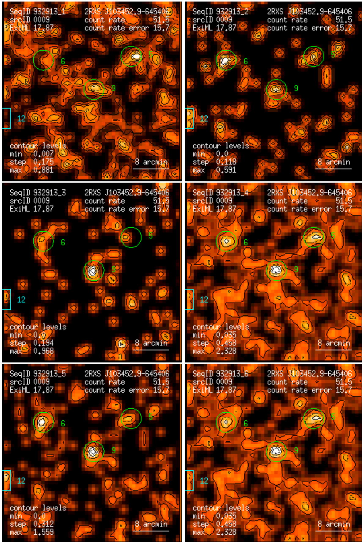
Figure 9: RASS 932913: detection 0009: band rate images, Gaussian filter: (1) PSPC channels 11 – 41, (2) 52 – 90, (3) 91 – 201, (4) 11 – 235, (5) 52 – 201, (6) 11 – 201. Broad band rates in counts/ks. Band rate contour levels in counts/ks/arcmin 2 .
