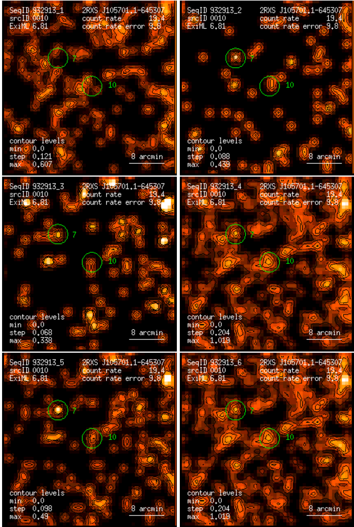
Figure 10: RASS 932913: detection 0010: band rate images, Gaussian filter: (1) PSPC channels 11 – 41, (2) 52 – 90, (3) 91 – 201, (4) 11 – 235, (5) 52 – 201, (6) 11 – 201. Broad band rates in counts/ks. Band rate contour levels in counts/ks/arcmin 2 .
