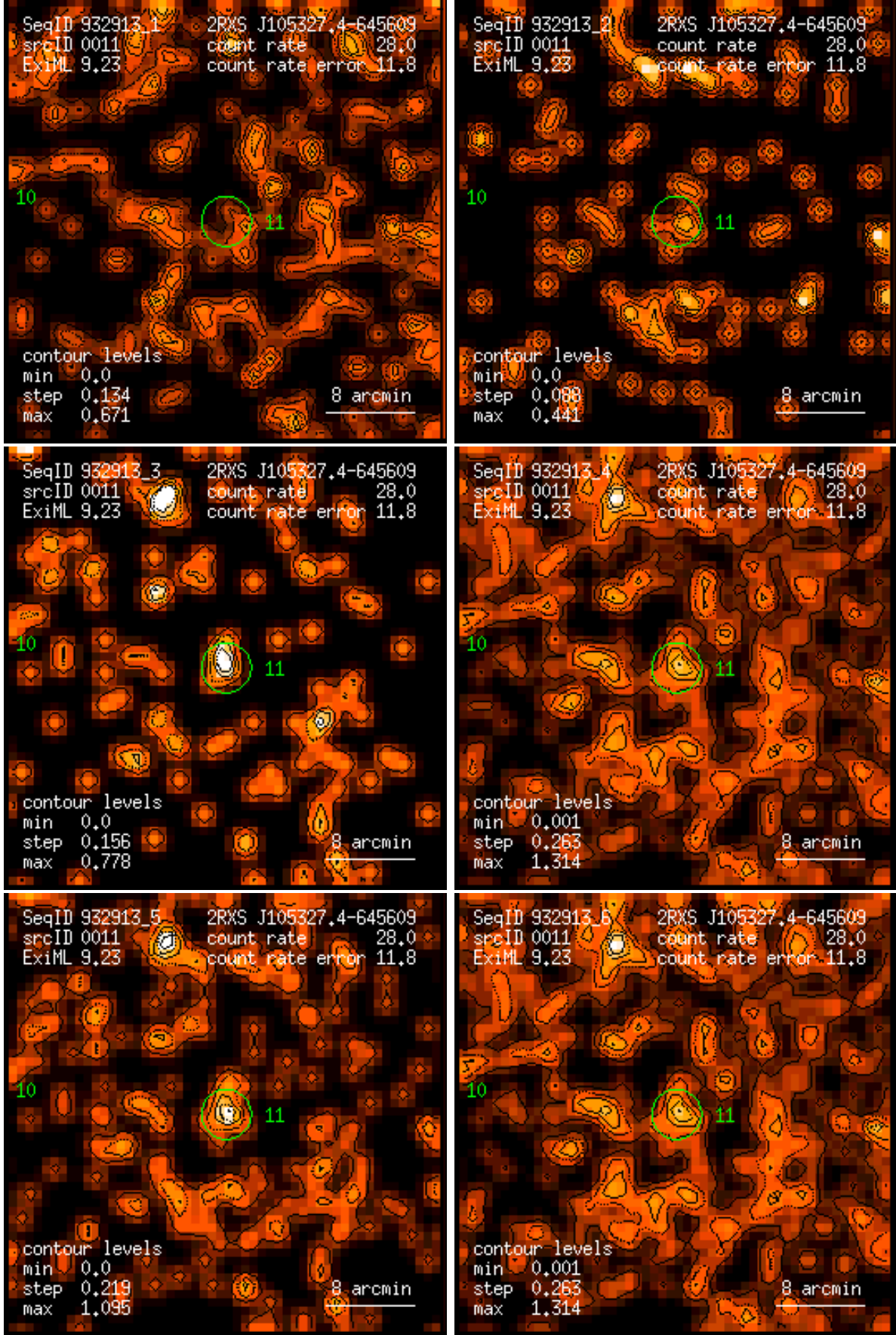
Figure 11: RASS 932913: detection 0011: band rate images, Gaussian filter: (1) PSPC channels 11 – 41, (2) 52 – 90, (3) 91 – 201, (4) 11 – 235, (5) 52 – 201, (6) 11 – 201. Broad band rates in counts/ks. Band rate contour levels in counts/ks/arcmin 2 .
