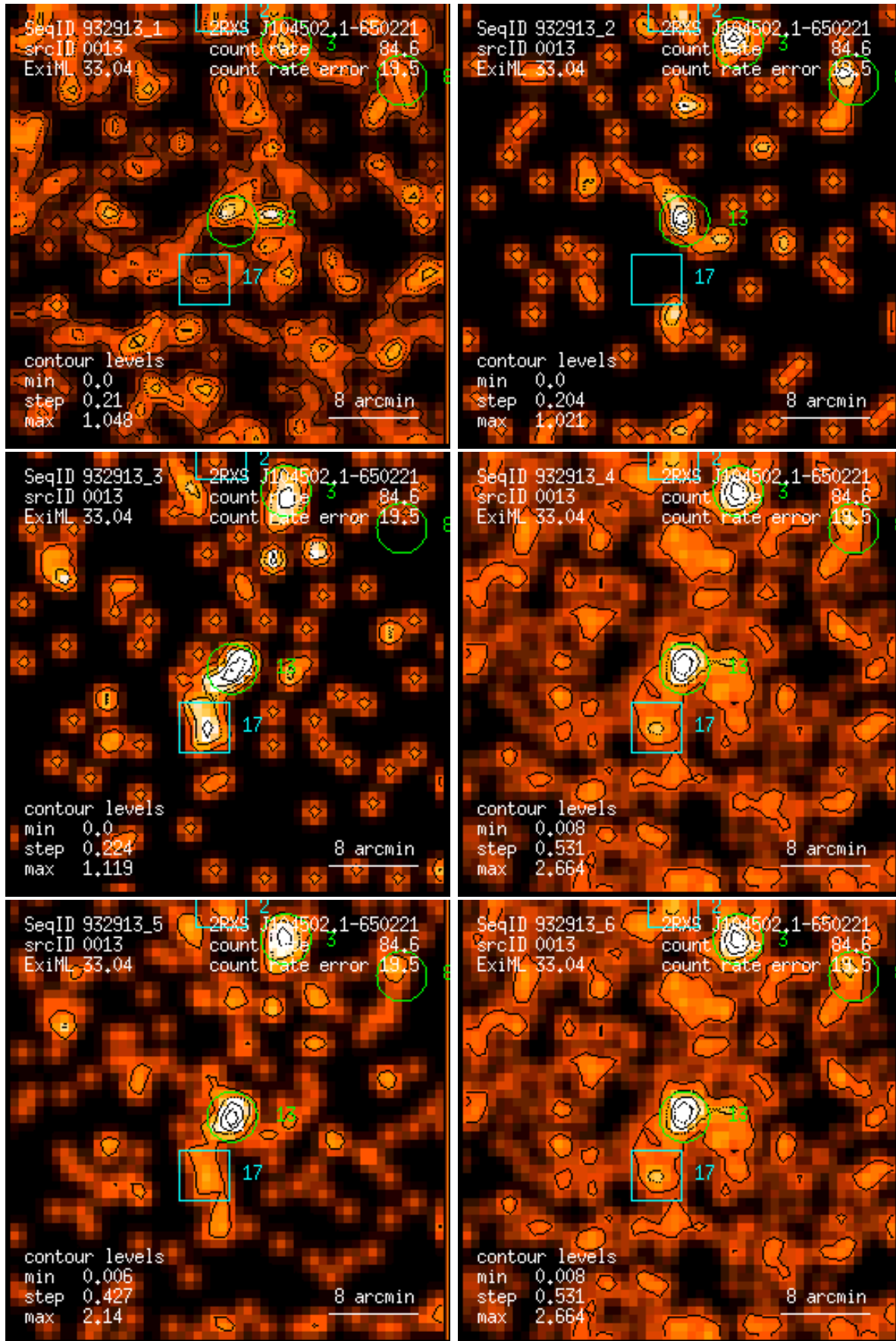
Figure 13: RASS 932913: detection 0013: band rate images, Gaussian filter: (1) PSPC channels 11 – 41, (2) 52 – 90, (3) 91 – 201, (4) 11 – 235, (5) 52 – 201, (6) 11 – 201. Broad band rates in counts/ks. Band rate contour levels in counts/ks/arcmin 2 .
