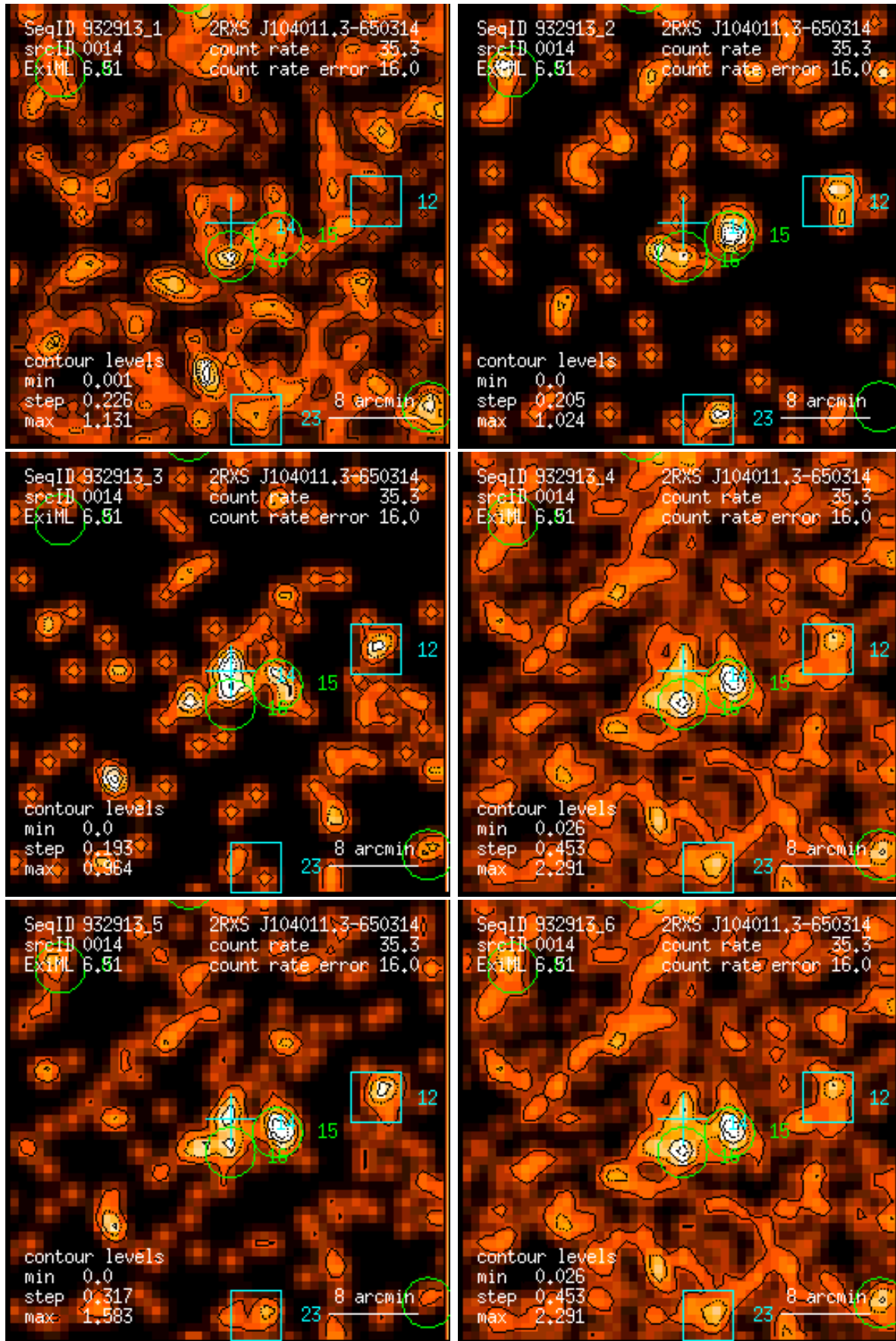
Figure 14: RASS 932913: detection 0014: band rate images, Gaussian filter: (1) PSPC channels 11 – 41, (2) 52 – 90, (3) 91 – 201, (4) 11 – 235, (5) 52 – 201, (6) 11 – 201. Broad band rates in counts/ks. Band rate contour levels in counts/ks/arcmin 2 .
