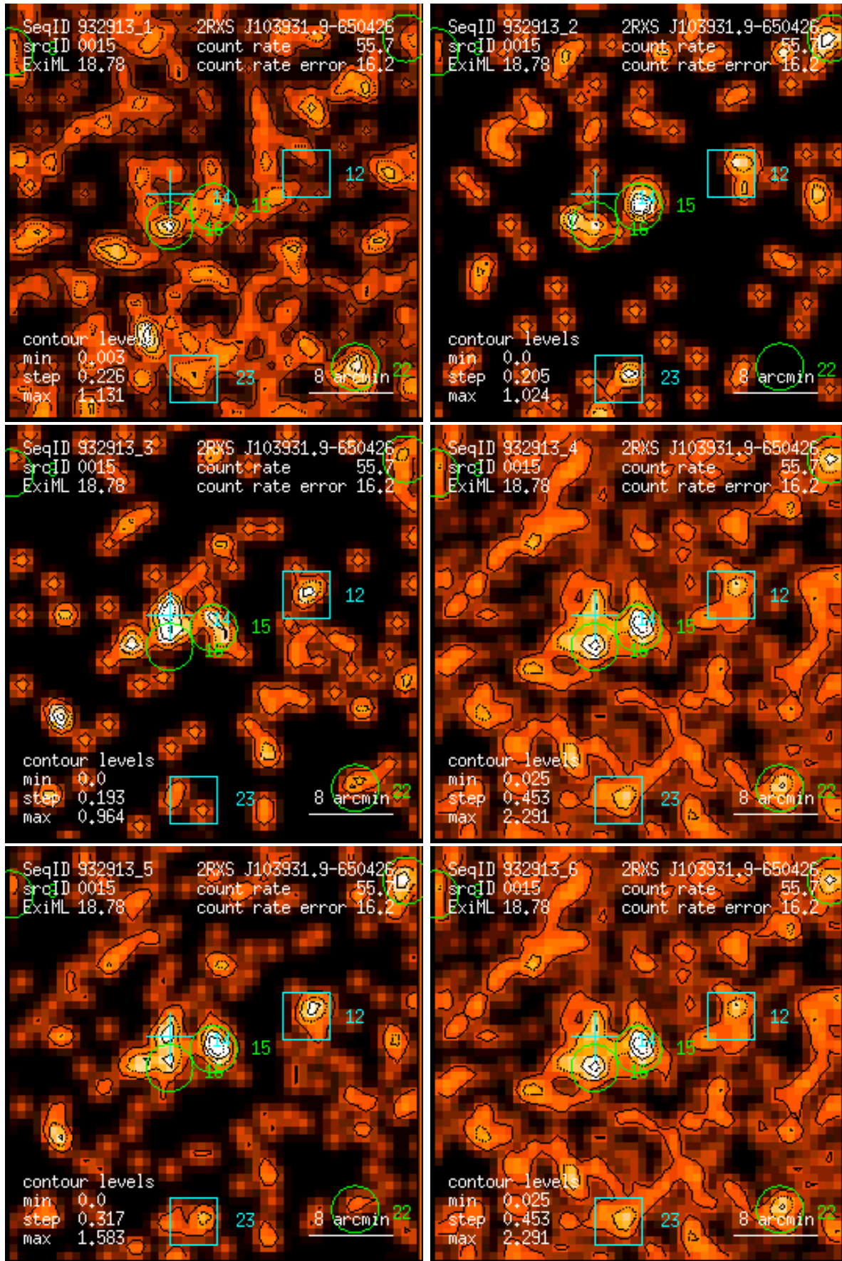
Figure 15: RASS 932913: detection 0015: band rate images, Gaussian filter: (1) PSPC channels 11 – 41, (2) 52 – 90, (3) 91 – 201, (4) 11 – 235, (5) 52 – 201, (6) 11 – 201. Broad band rates in counts/ks. Band rate contour levels in counts/ks/arcmin 2 .
