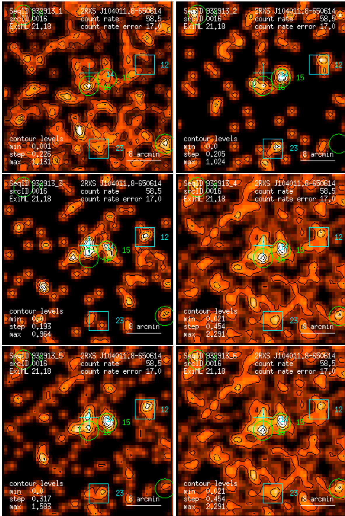
Figure 16: RASS 932913: detection 0016: band rate images, Gaussian filter: (1) PSPC channels 11 – 41, (2) 52 – 90, (3) 91 – 201, (4) 11 – 235, (5) 52 – 201, (6) 11 – 201. Broad band rates in counts/ks. Band rate contour levels in counts/ks/arcmin 2 .
