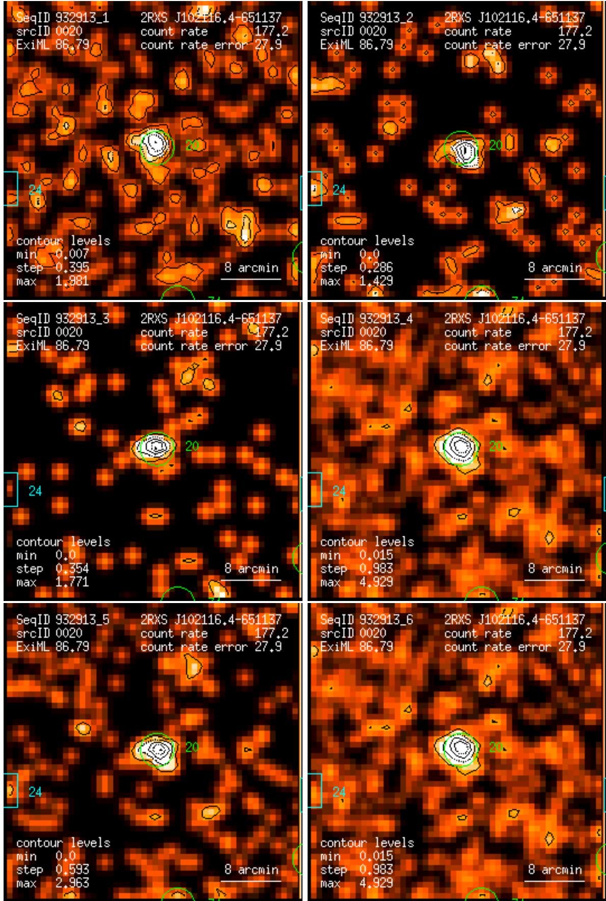
Figure 20: RASS 932913: detection 0020: band rate images, Gaussian filter: (1) PSPC channels 11 – 41, (2) 52 – 90, (3) 91 – 201, (4) 11 – 235, (5) 52 – 201, (6) 11 – 201. Broad band rates in counts/ks. Band rate contour levels in counts/ks/arcmin 2 .
