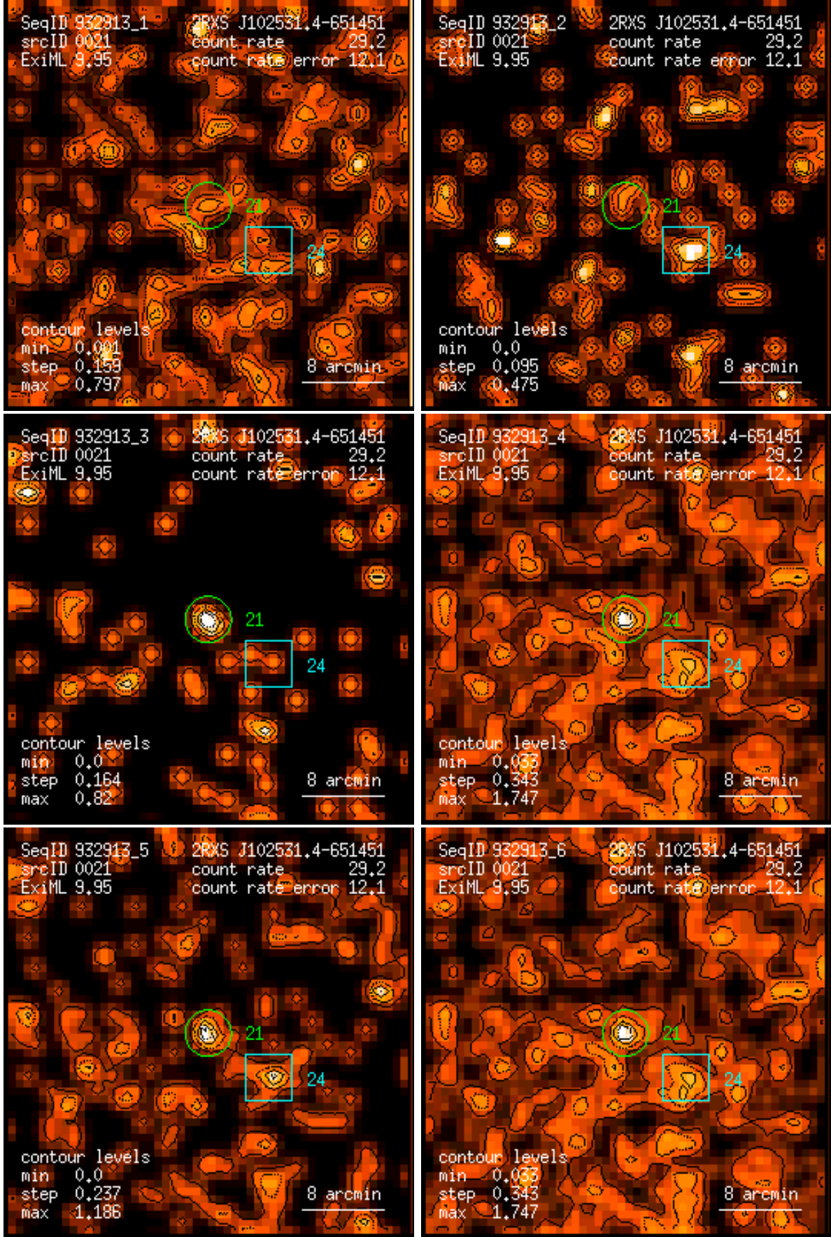
Figure 21: RASS 932913: detection 0021: band rate images, Gaussian filter: (1) PSPC channels 11 – 41, (2) 52 – 90, (3) 91 – 201, (4) 11 – 235, (5) 52 – 201, (6) 11 – 201. Broad band rates in counts/ks. Band rate contour levels in counts/ks/arcmin 2 .
