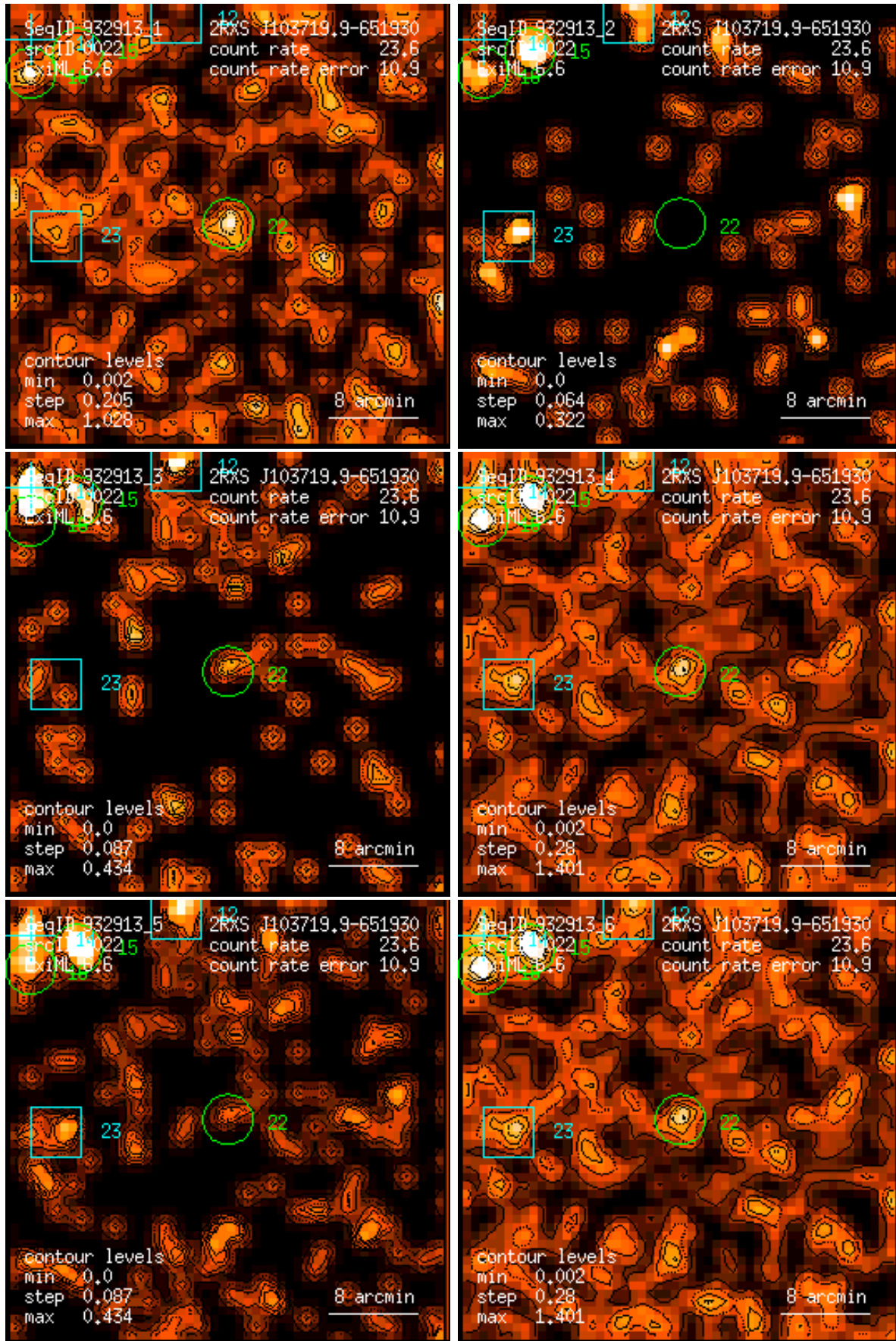
Figure 22: RASS 932913: detection 0022: band rate images, Gaussian filter: (1) PSPC channels 11 – 41, (2) 52 – 90, (3) 91 – 201, (4) 11 – 235, (5) 52 – 201, (6) 11 – 201. Broad band rates in counts/ks. Band rate contour levels in counts/ks/arcmin 2 .
