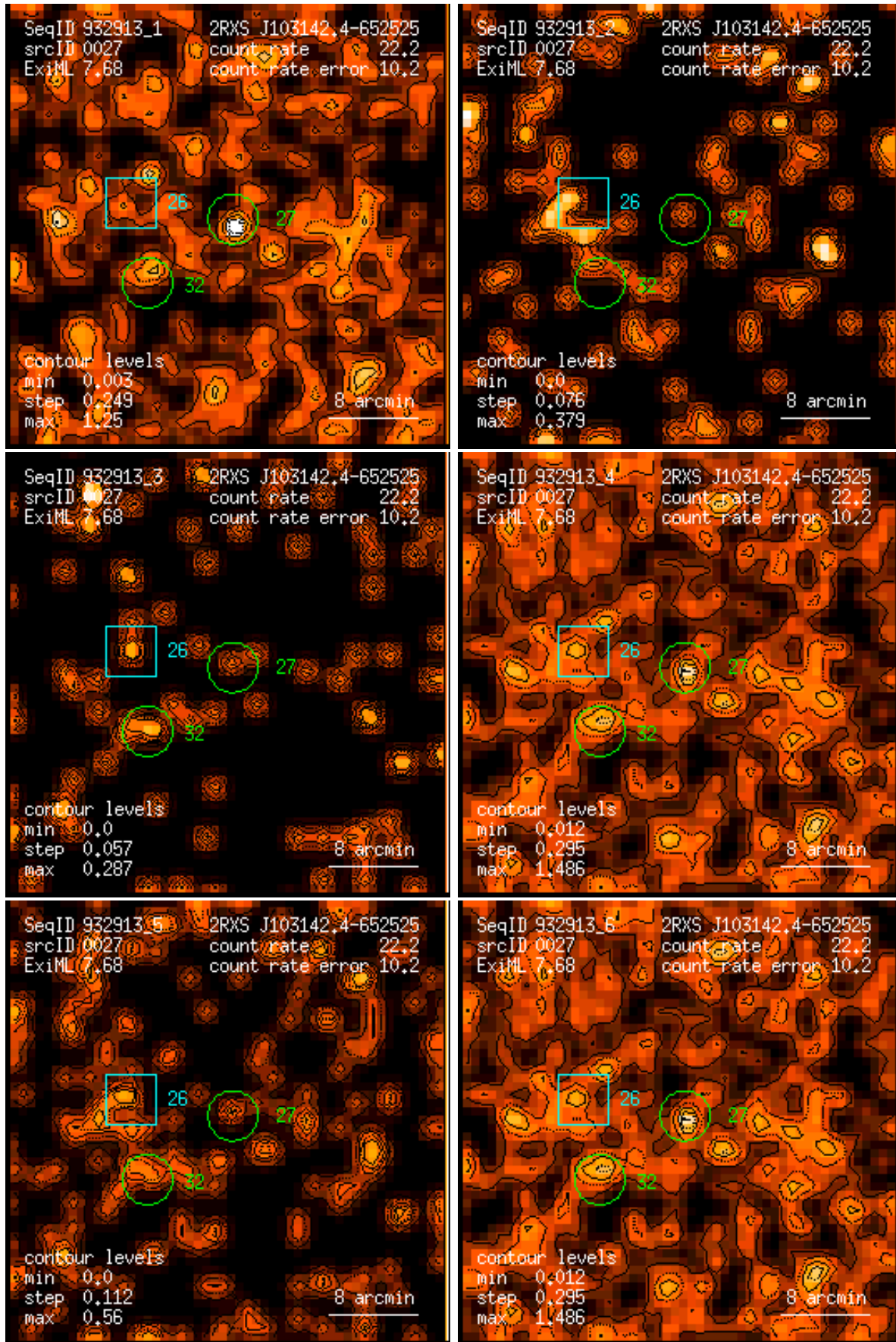
Figure 27: RASS 932913: detection 0027: band rate images, Gaussian filter: (1) PSPC channels 11 – 41, (2) 52 – 90, (3) 91 – 201, (4) 11 – 235, (5) 52 – 201, (6) 11 – 201. Broad band rates in counts/ks. Band rate contour levels in counts/ks/arcmin 2 .
