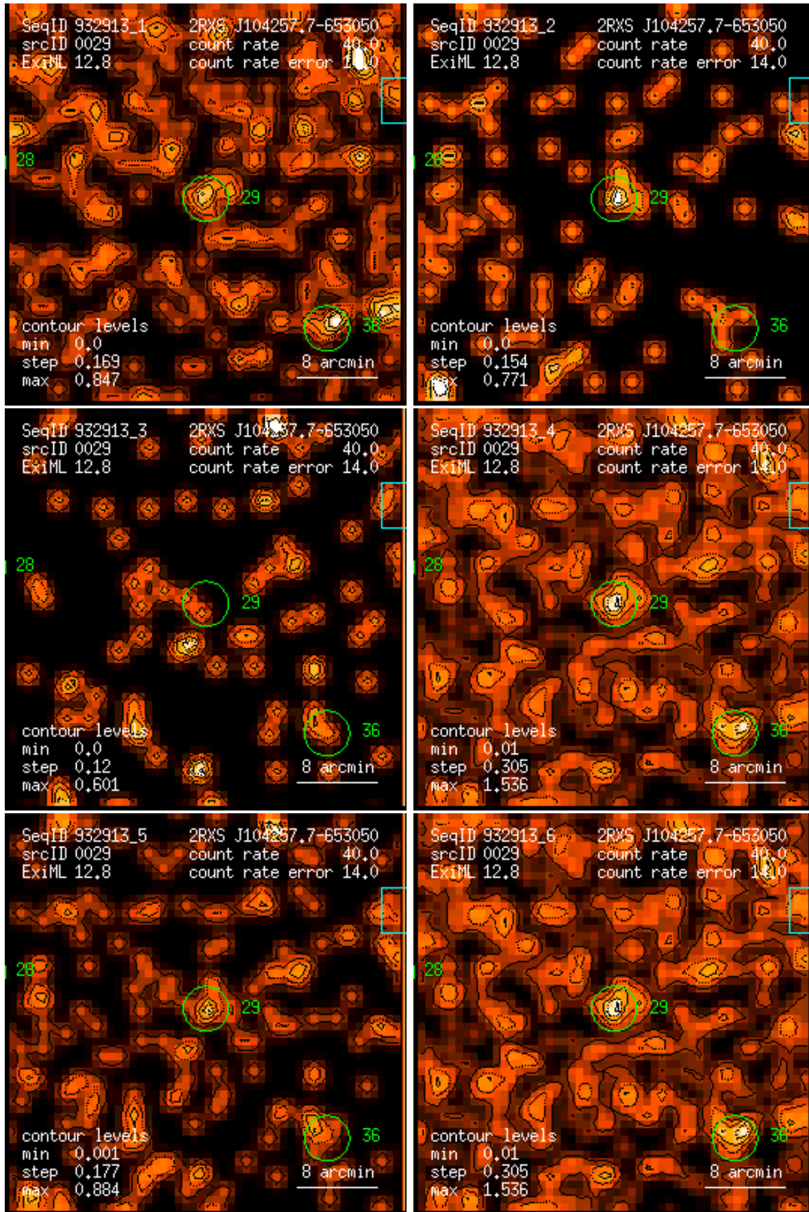
Figure 29: RASS 932913: detection 0029: band rate images, Gaussian filter: (1) PSPC channels 11 – 41, (2) 52 – 90, (3) 91 – 201, (4) 11 – 235, (5) 52 – 201, (6) 11 – 201. Broad band rates in counts/ks. Band rate contour levels in counts/ks/arcmin 2 .
