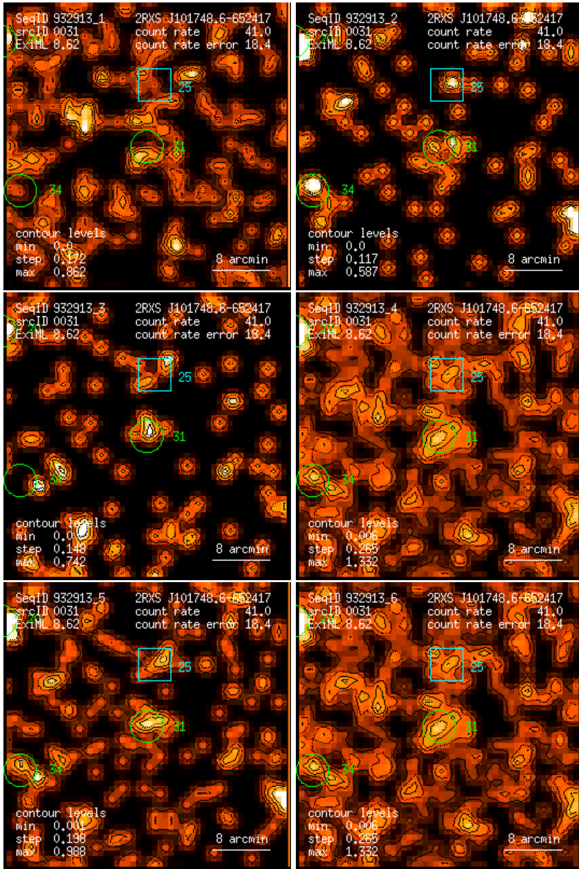
Figure 31: RASS 932913: detection 0031: band rate images, Gaussian filter: (1) PSPC channels 11 – 41, (2) 52 – 90, (3) 91 – 201, (4) 11 – 235, (5) 52 – 201, (6) 11 – 201. Broad band rates in counts/ks. Band rate contour levels in counts/ks/arcmin 2 .
