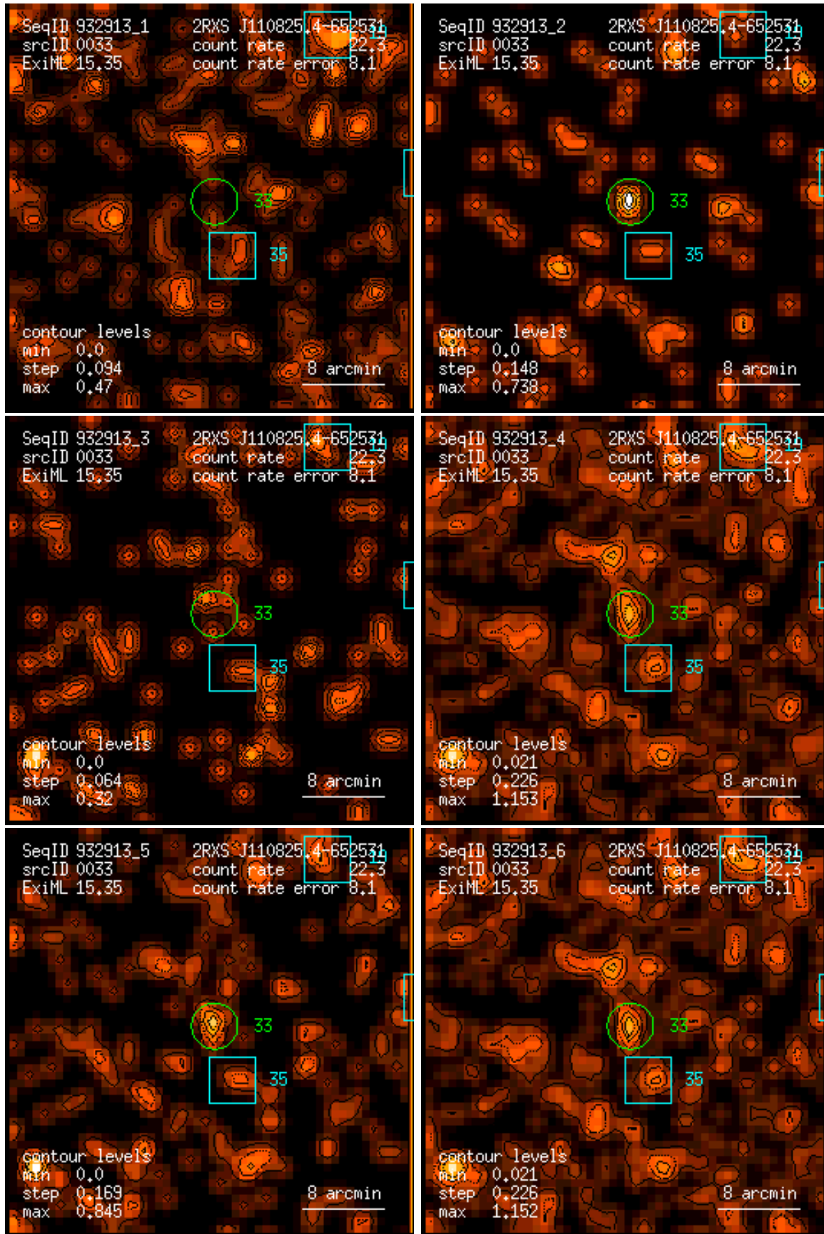
Figure 33: RASS 932913: detection 0033: band rate images, Gaussian filter: (1) PSPC channels 11 – 41, (2) 52 – 90, (3) 91 – 201, (4) 11 – 235, (5) 52 – 201, (6) 11 – 201. Broad band rates in counts/ks. Band rate contour levels in counts/ks/arcmin 2 .
