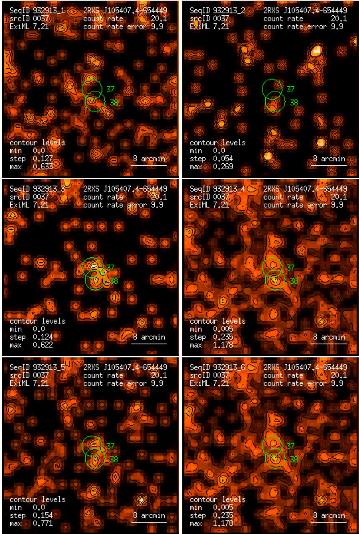
Figure 37: RASS 932913: detection 0037: band rate images, Gaussian filter: (1) PSPC channels 11 – 41, (2) 52 – 90, (3) 91 – 201, (4) 11 – 235, (5) 52 – 201, (6) 11 – 201. Broad band rates in counts/ks. Band rate contour levels in counts/ks/arcmin 2 .
