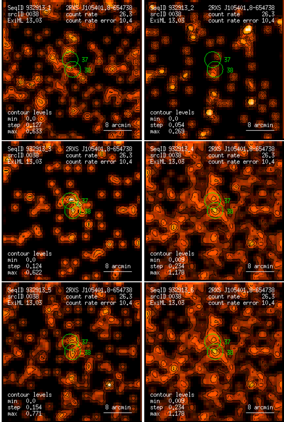
Figure 38: RASS 932913: detection 0038: band rate images, Gaussian filter: (1) PSPC channels 11 – 41, (2) 52 – 90, (3) 91 – 201, (4) 11 – 235, (5) 52 – 201, (6) 11 – 201. Broad band rates in counts/ks. Band rate contour levels in counts/ks/arcmin 2 .
