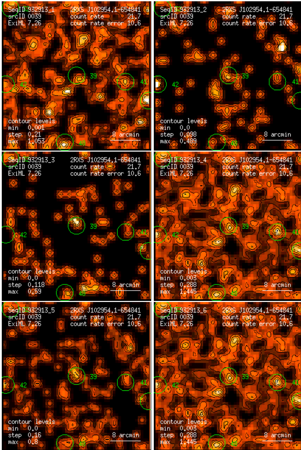
Figure 39: RASS 932913: detection 0039: band rate images, Gaussian filter: (1) PSPC channels 11 – 41, (2) 52 – 90, (3) 91 – 201, (4) 11 – 235, (5) 52 – 201, (6) 11 – 201. Broad band rates in counts/ks. Band rate contour levels in counts/ks/arcmin 2 .
