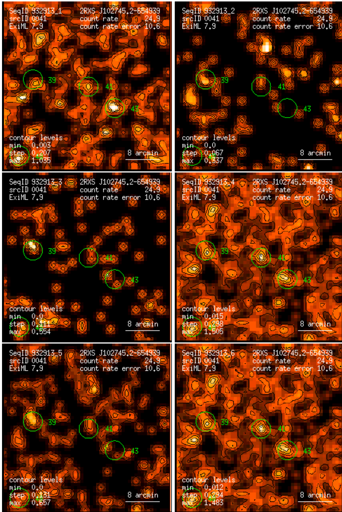
Figure 41: RASS 932913: detection 0041: band rate images, Gaussian filter: (1) PSPC channels 11 – 41, (2) 52 – 90, (3) 91 – 201, (4) 11 – 235, (5) 52 – 201, (6) 11 – 201. Broad band rates in counts/ks. Band rate contour levels in counts/ks/arcmin 2 .
