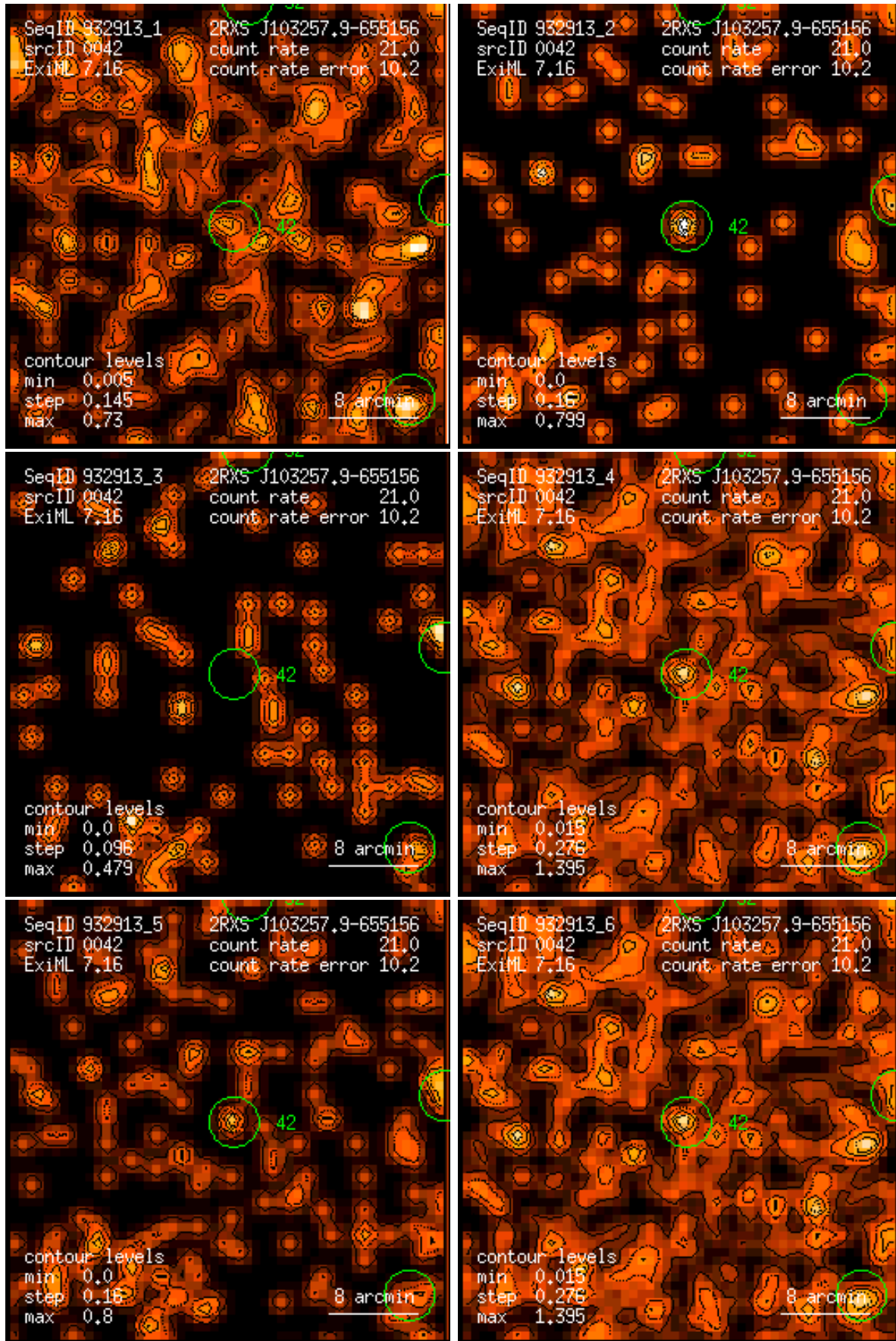
Figure 42: RASS 932913: detection 0042: band rate images, Gaussian filter: (1) PSPC channels 11 – 41, (2) 52 – 90, (3) 91 – 201, (4) 11 – 235, (5) 52 – 201, (6) 11 – 201. Broad band rates in counts/ks. Band rate contour levels in counts/ks/arcmin 2 .
