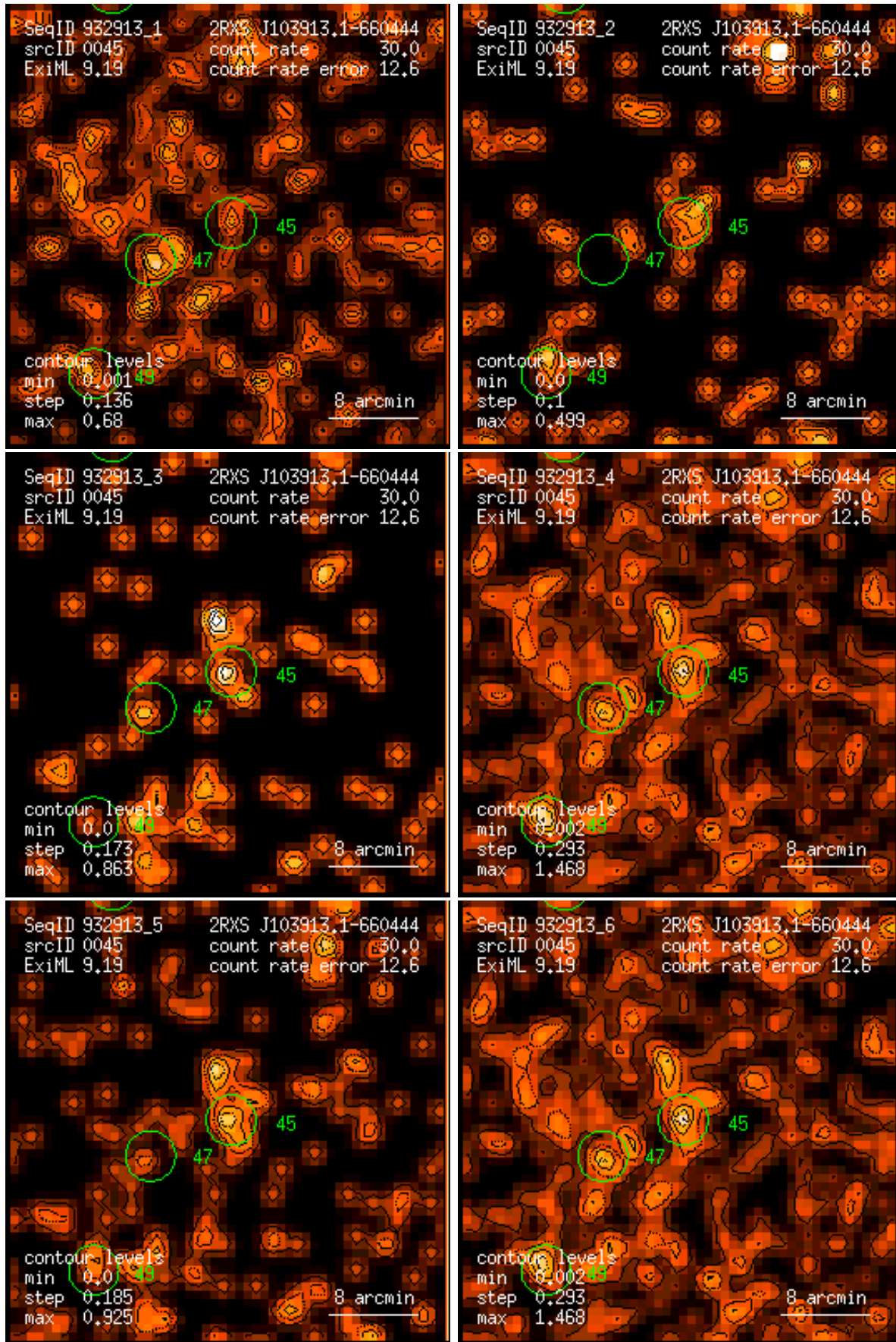
Figure 45: RASS 932913: detection 0045: band rate images, Gaussian filter: (1) PSPC channels 11 – 41, (2) 52 – 90, (3) 91 – 201, (4) 11 – 235, (5) 52 – 201, (6) 11 – 201. Broad band rates in counts/ks. Band rate contour levels in counts/ks/arcmin 2 .
