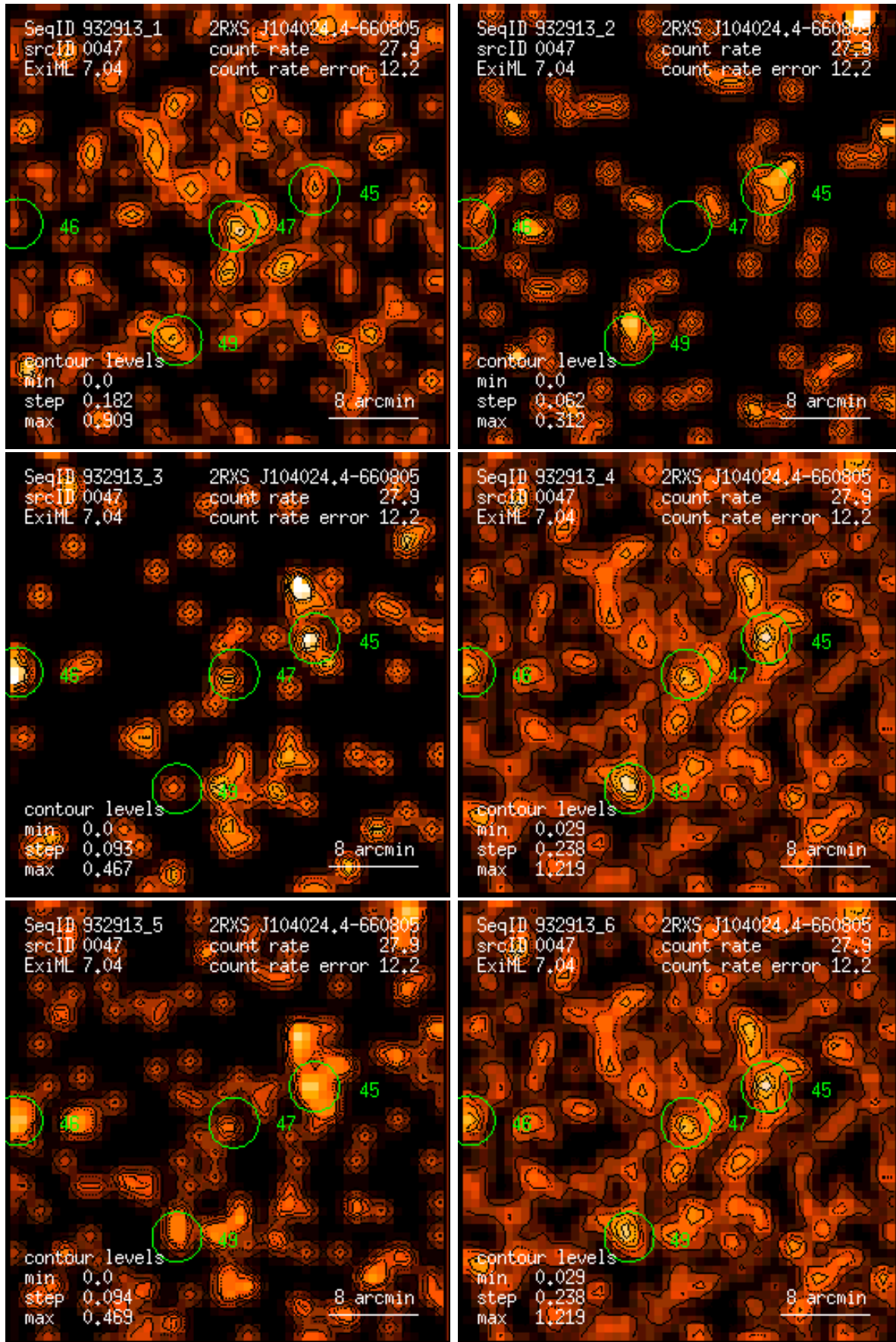
Figure 47: RASS 932913: detection 0047: band rate images, Gaussian filter: (1) PSPC channels 11 – 41, (2) 52 – 90, (3) 91 – 201, (4) 11 – 235, (5) 52 – 201, (6) 11 – 201. Broad band rates in counts/ks. Band rate contour levels in counts/ks/arcmin 2 .
