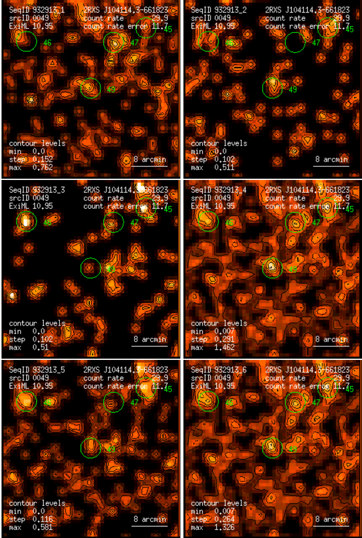
Figure 49: RASS 932913: detection 0049: band rate images, Gaussian filter: (1) PSPC channels 11 – 41, (2) 52 – 90, (3) 91 – 201, (4) 11 – 235, (5) 52 – 201, (6) 11 – 201. Broad band rates in counts/ks. Band rate contour levels in counts/ks/arcmin 2 .
