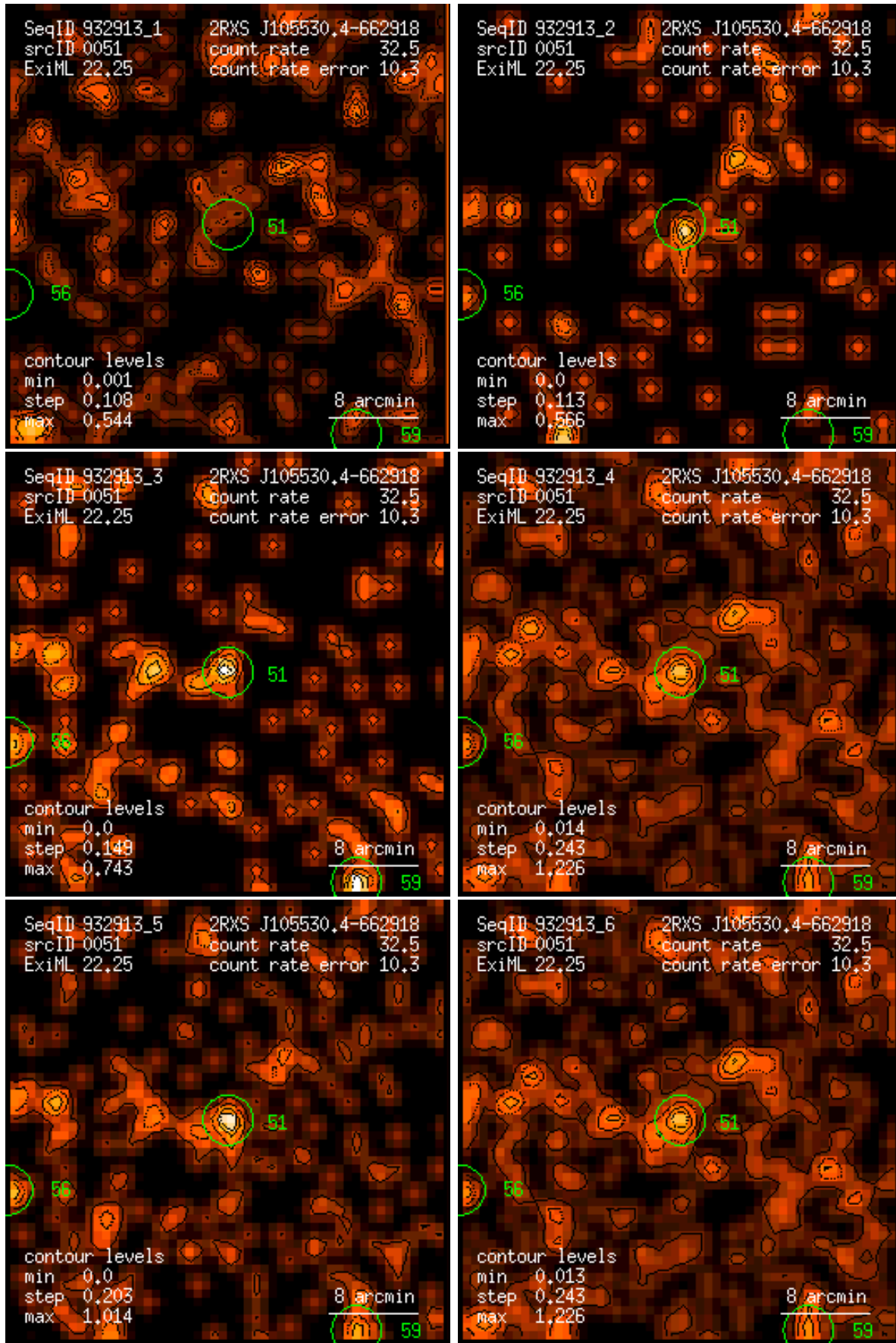
Figure 51: RASS 932913: detection 0051: band rate images, Gaussian filter: (1) PSPC channels 11 – 41, (2) 52 – 90, (3) 91 – 201, (4) 11 – 235, (5) 52 – 201, (6) 11 – 201. Broad band rates in counts/ks. Band rate contour levels in counts/ks/arcmin 2 .
