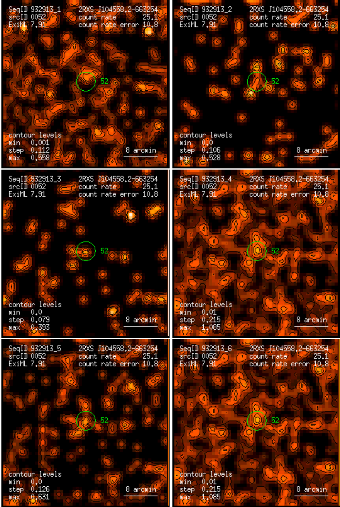
Figure 52: RASS 932913: detection 0052: band rate images, Gaussian filter: (1) PSPC channels 11 – 41, (2) 52 – 90, (3) 91 – 201, (4) 11 – 235, (5) 52 – 201, (6) 11 – 201. Broad band rates in counts/ks. Band rate contour levels in counts/ks/arcmin 2 .
