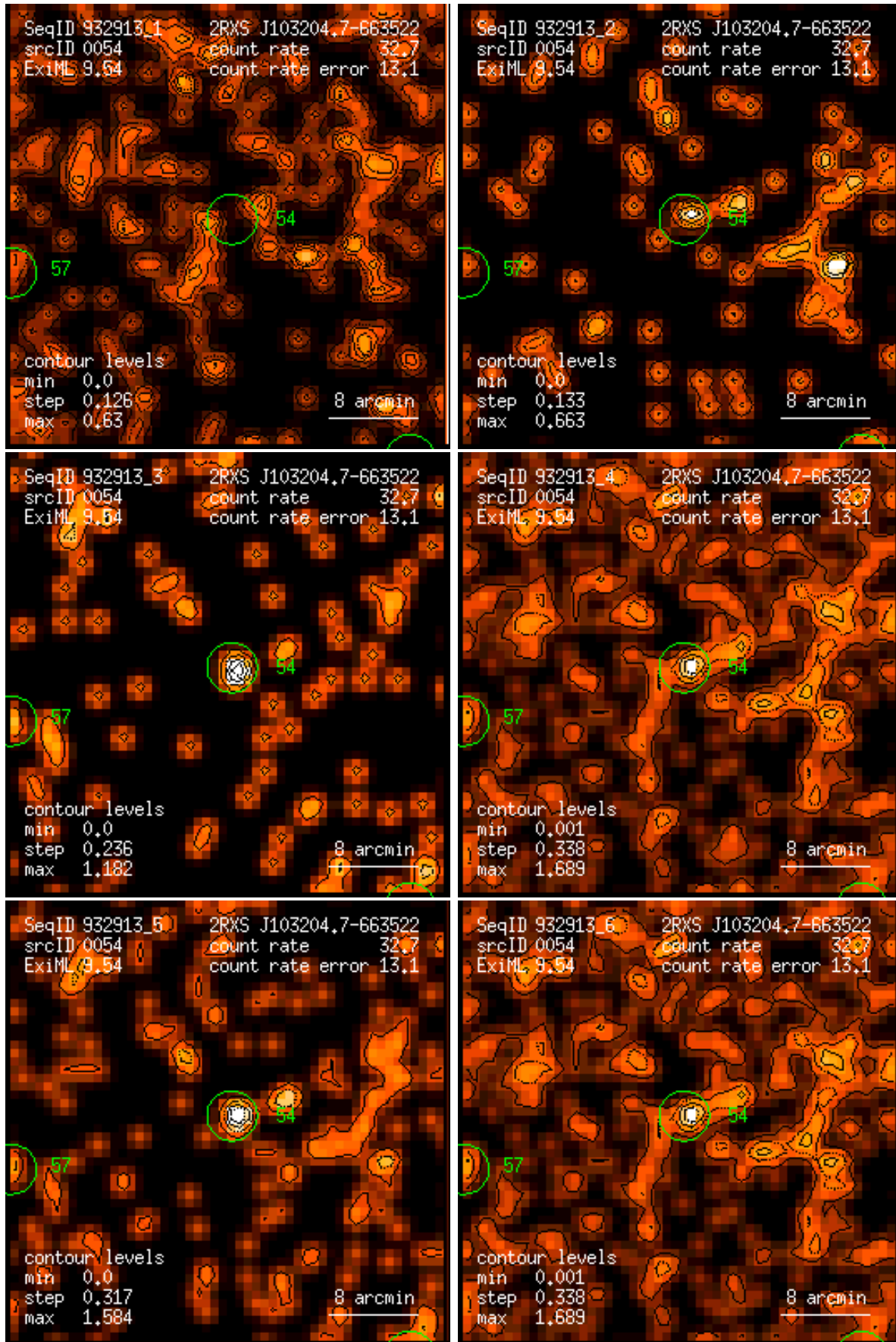
Figure 54: RASS 932913: detection 0054: band rate images, Gaussian filter: (1) PSPC channels 11 – 41, (2) 52 – 90, (3) 91 – 201, (4) 11 – 235, (5) 52 – 201, (6) 11 – 201. Broad band rates in counts/ks. Band rate contour levels in counts/ks/arcmin 2 .
