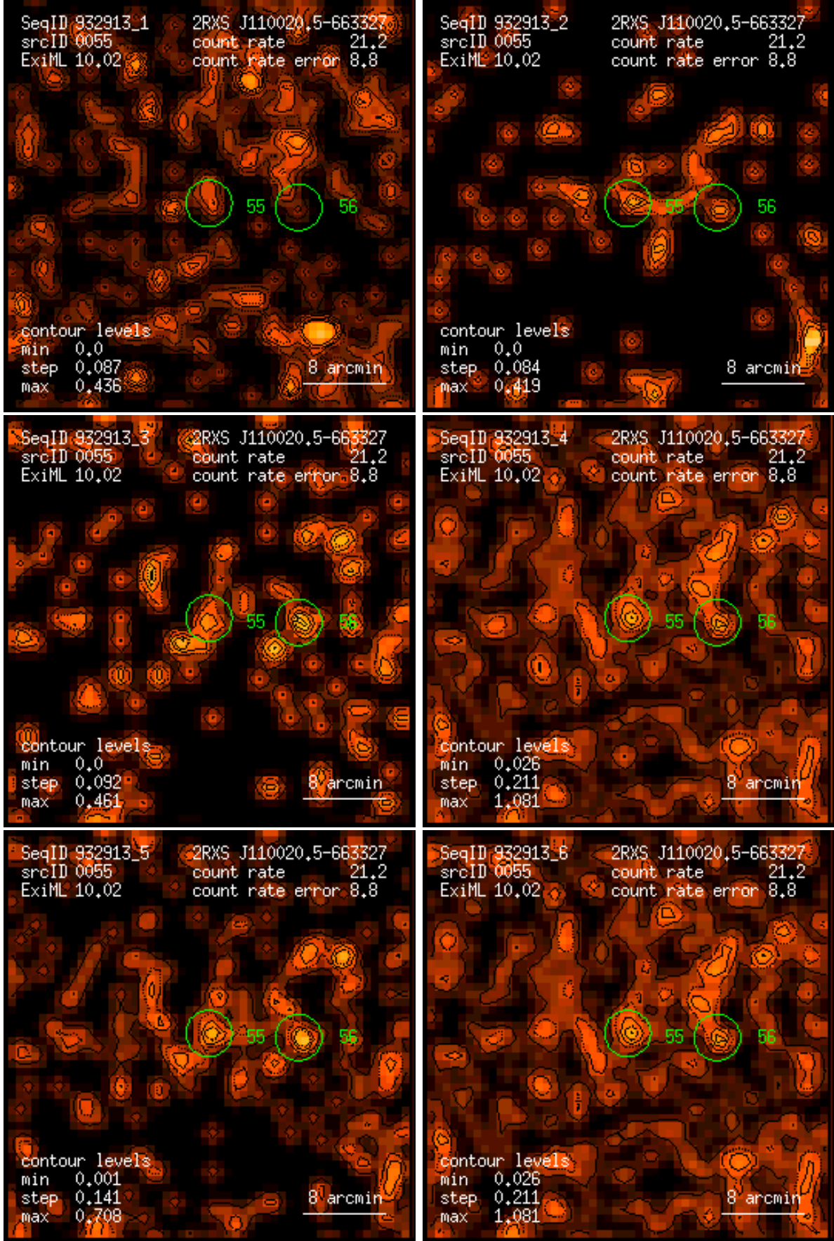
Figure 55: RASS 932913: detection 0055: band rate images, Gaussian filter: (1) PSPC channels 11 – 41, (2) 52 – 90, (3) 91 – 201, (4) 11 – 235, (5) 52 – 201, (6) 11 – 201. Broad band rates in counts/ks. Band rate contour levels in counts/ks/arcmin 2 .
