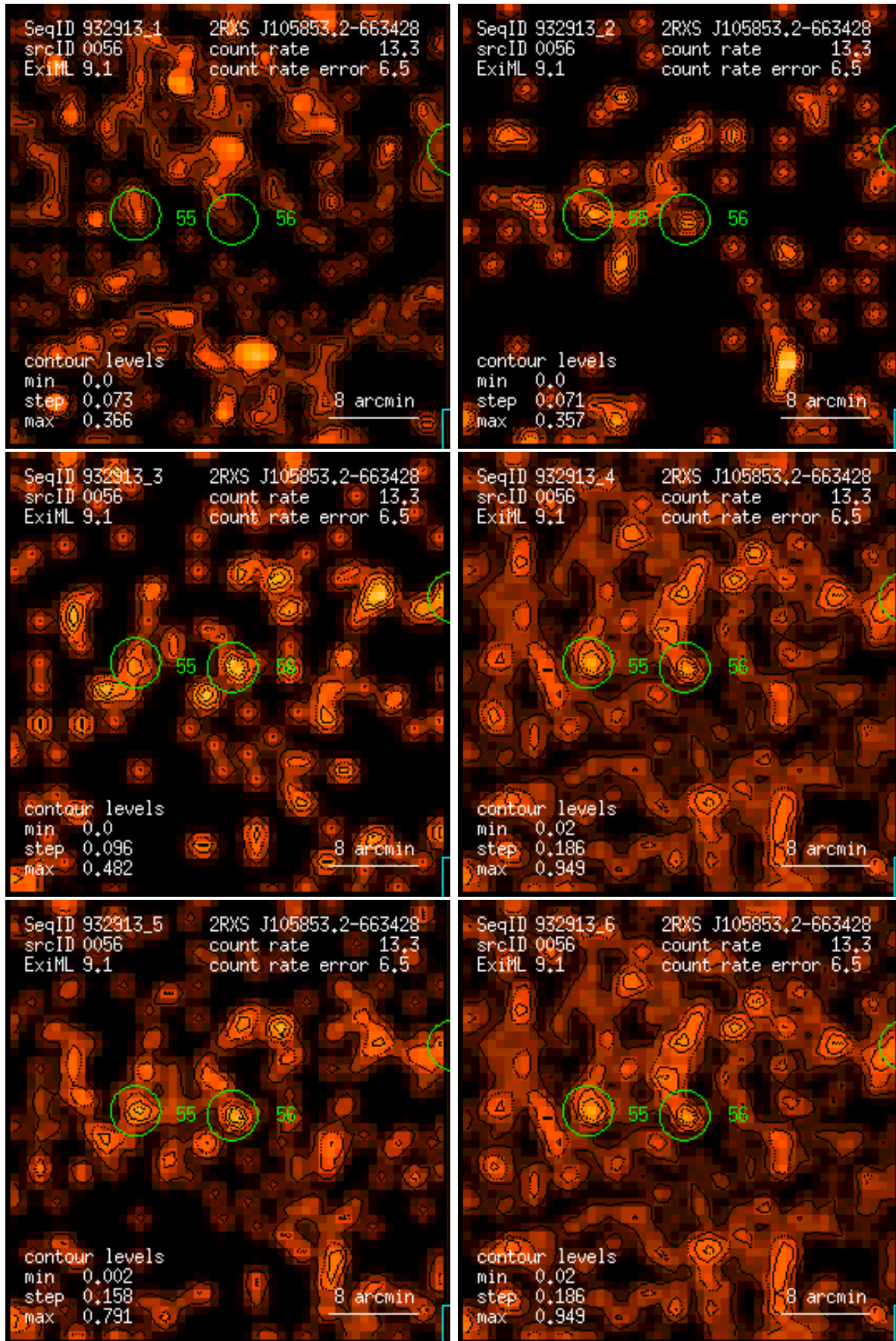
Figure 56: RASS 932913: detection 0056: band rate images, Gaussian filter: (1) PSPC channels 11 – 41, (2) 52 – 90, (3) 91 – 201, (4) 11 – 235, (5) 52 – 201, (6) 11 – 201. Broad band rates in counts/ks. Band rate contour levels in counts/ks/arcmin 2 .
