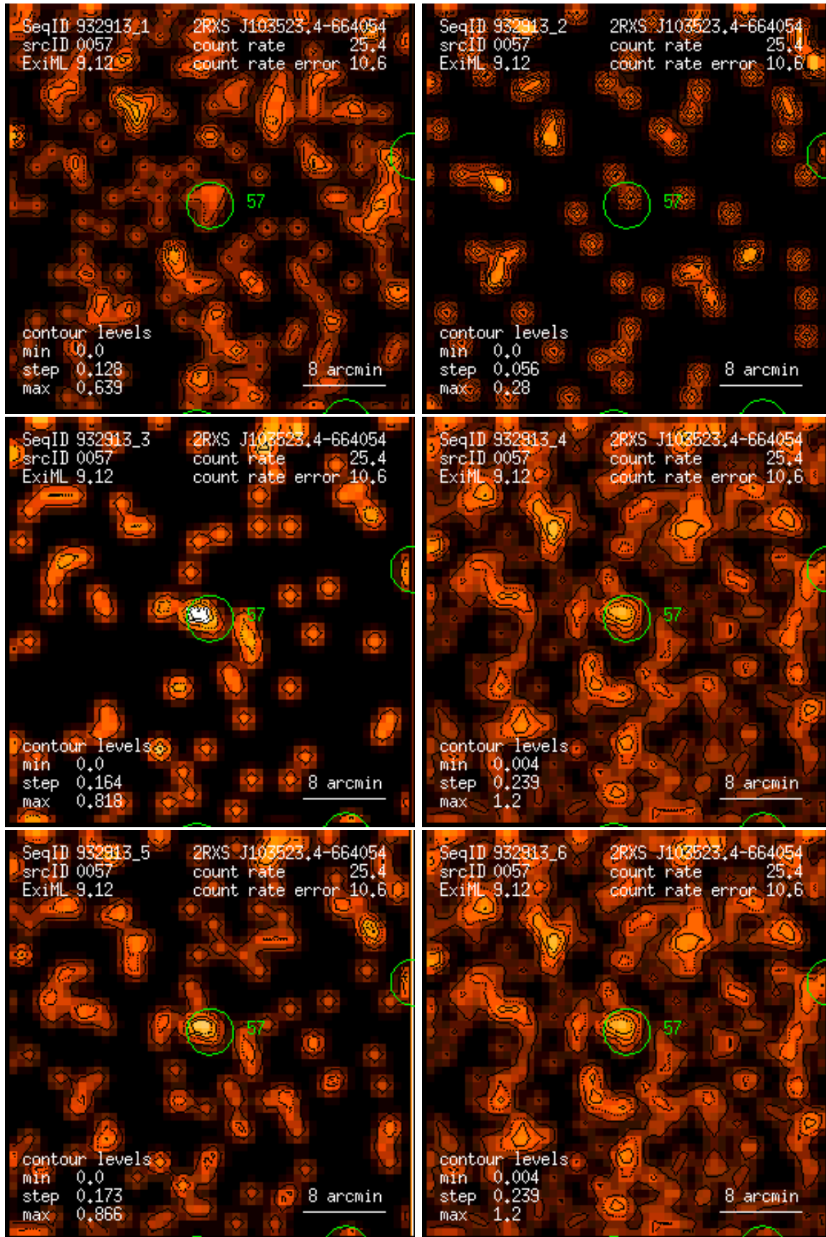
Figure 57: RASS 932913: detection 0057: band rate images, Gaussian filter: (1) PSPC channels 11 – 41, (2) 52 – 90, (3) 91 – 201, (4) 11 – 235, (5) 52 – 201, (6) 11 – 201. Broad band rates in counts/ks. Band rate contour levels in counts/ks/arcmin 2 .
