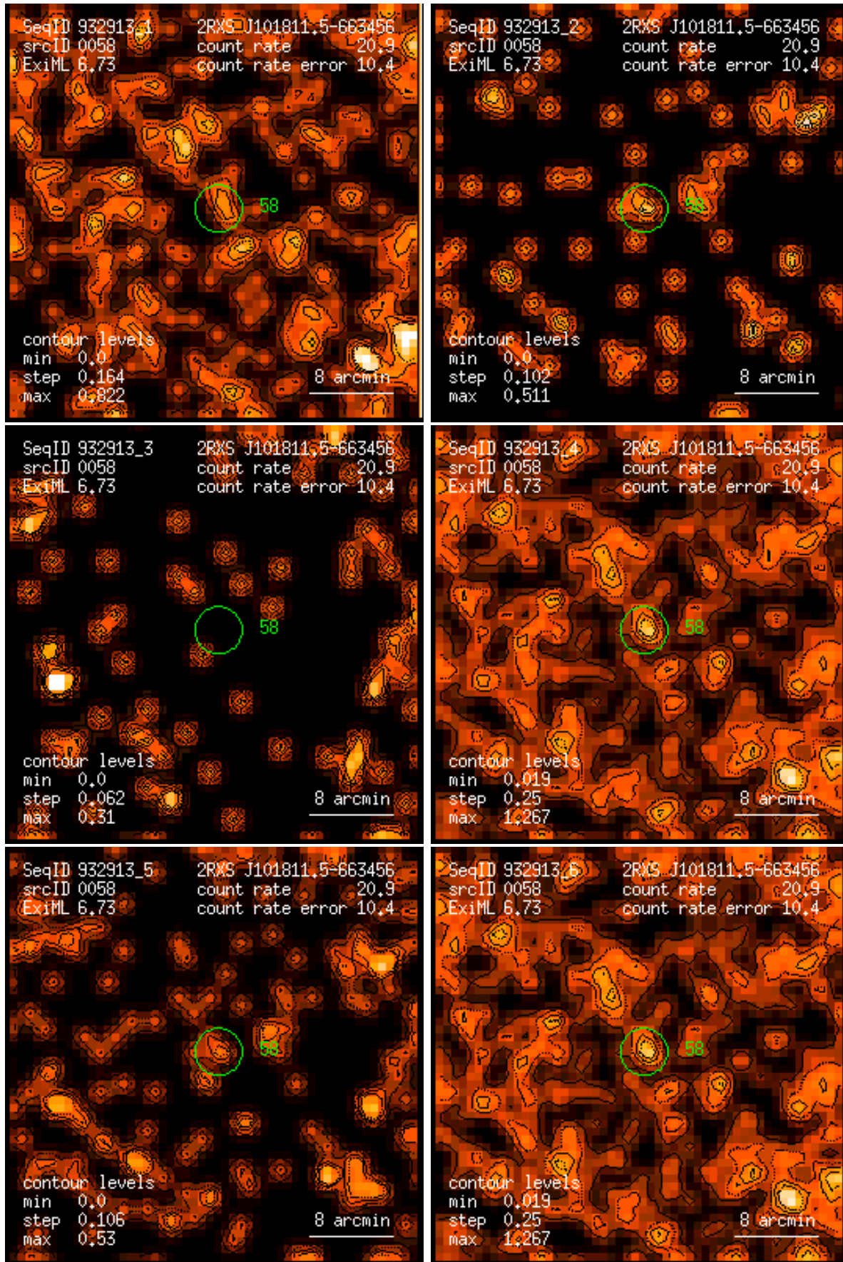
Figure 58: RASS 932913: detection 0058: band rate images, Gaussian filter: (1) PSPC channels 11 – 41, (2) 52 – 90, (3) 91 – 201, (4) 11 – 235, (5) 52 – 201, (6) 11 – 201. Broad band rates in counts/ks. Band rate contour levels in counts/ks/arcmin 2 .
