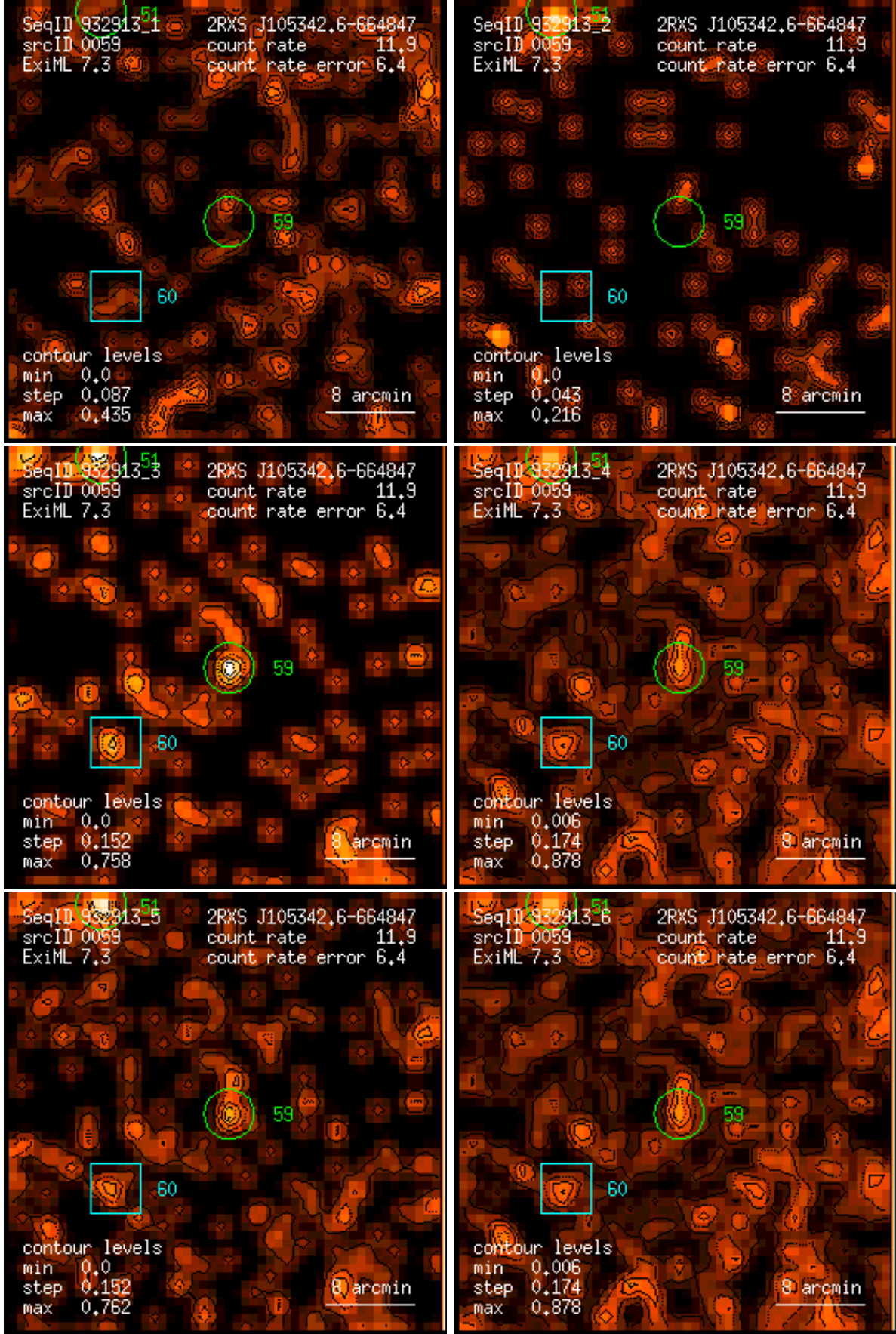
Figure 59: RASS 932913: detection 0059: band rate images, Gaussian filter: (1) PSPC channels 11 – 41, (2) 52 – 90, (3) 91 – 201, (4) 11 – 235, (5) 52 – 201, (6) 11 – 201. Broad band rates in counts/ks. Band rate contour levels in counts/ks/arcmin 2 .
