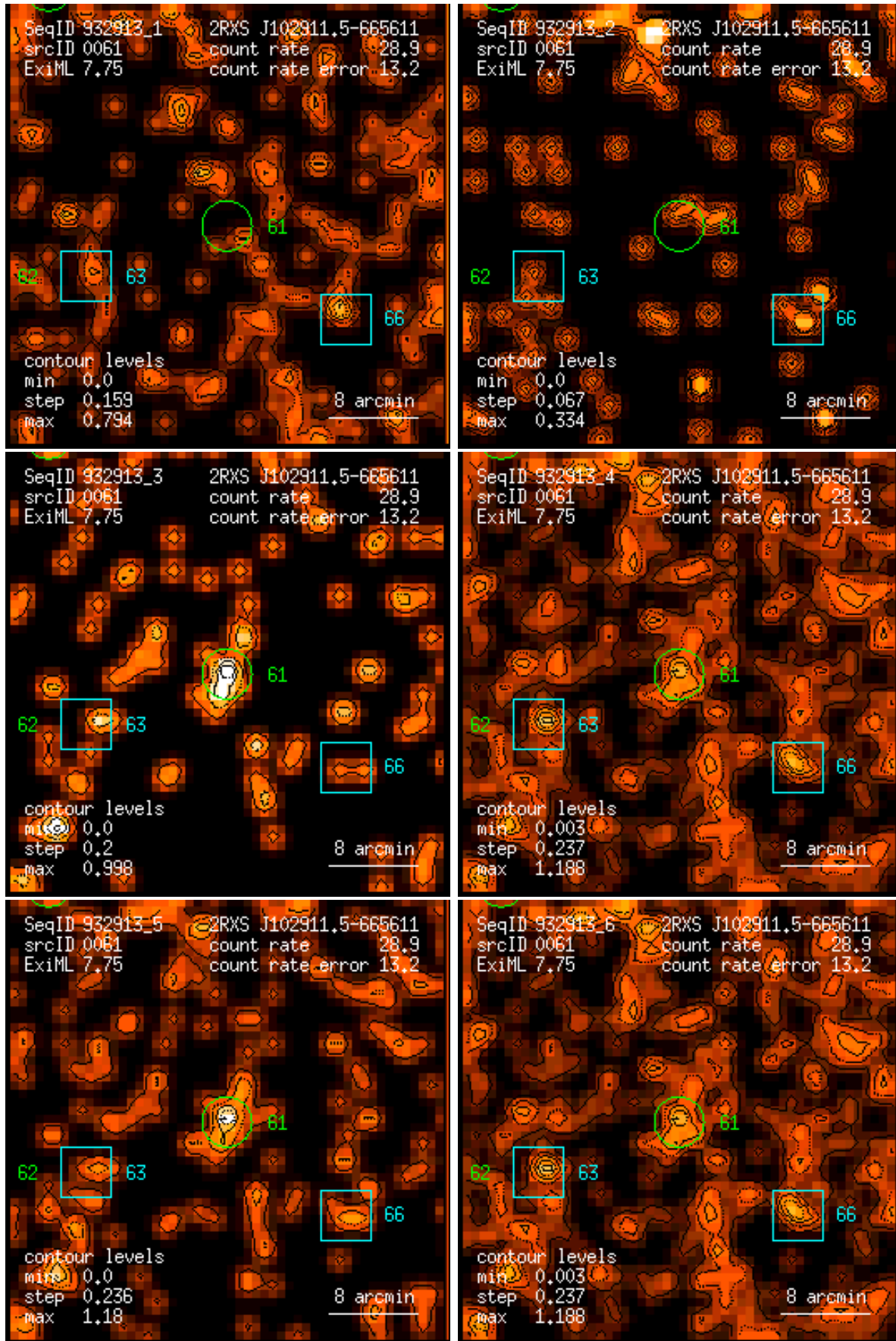
Figure 61: RASS 932913: detection 0061: band rate images, Gaussian filter: (1) PSPC channels 11 – 41, (2) 52 – 90, (3) 91 – 201, (4) 11 – 235, (5) 52 – 201, (6) 11 – 201. Broad band rates in counts/ks. Band rate contour levels in counts/ks/arcmin 2 .
