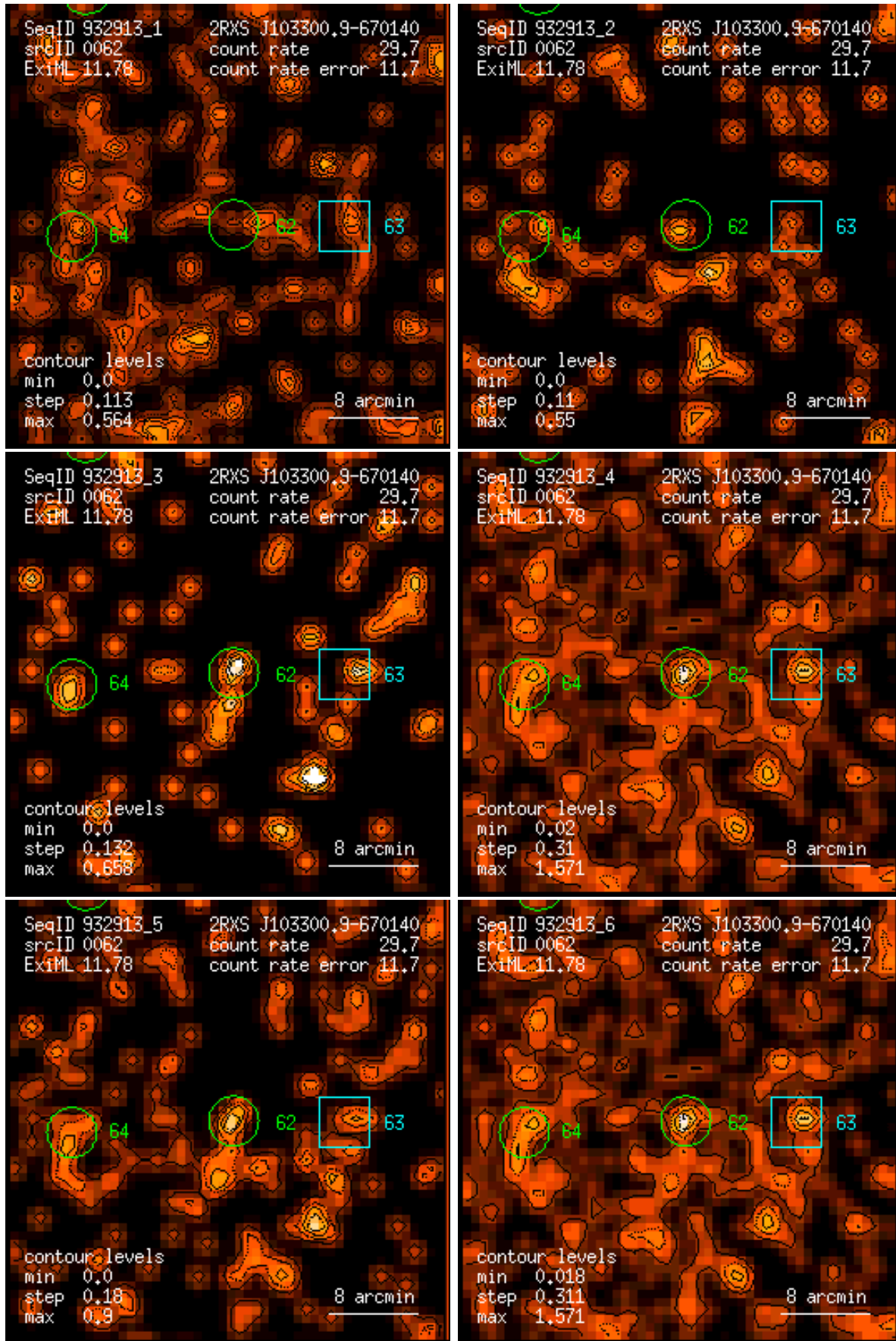
Figure 62: RASS 932913: detection 0062: band rate images, Gaussian filter: (1) PSPC channels 11 – 41, (2) 52 – 90, (3) 91 – 201, (4) 11 – 235, (5) 52 – 201, (6) 11 – 201. Broad band rates in counts/ks. Band rate contour levels in counts/ks/arcmin 2 .
