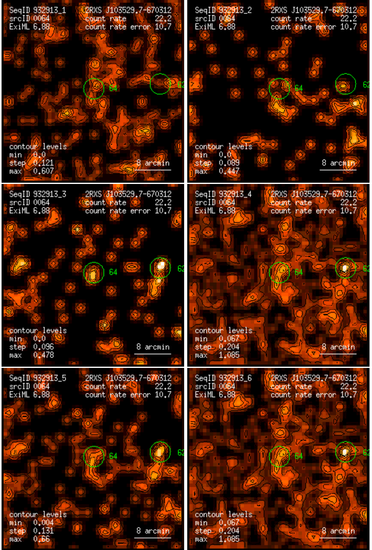
Figure 64: RASS 932913: detection 0064: band rate images, Gaussian filter: (1) PSPC channels 11 – 41, (2) 52 – 90, (3) 91 – 201, (4) 11 – 235, (5) 52 – 201, (6) 11 – 201. Broad band rates in counts/ks. Band rate contour levels in counts/ks/arcmin 2 .
